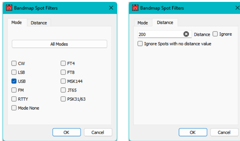
Figure 174 – Bandmap Filter options
