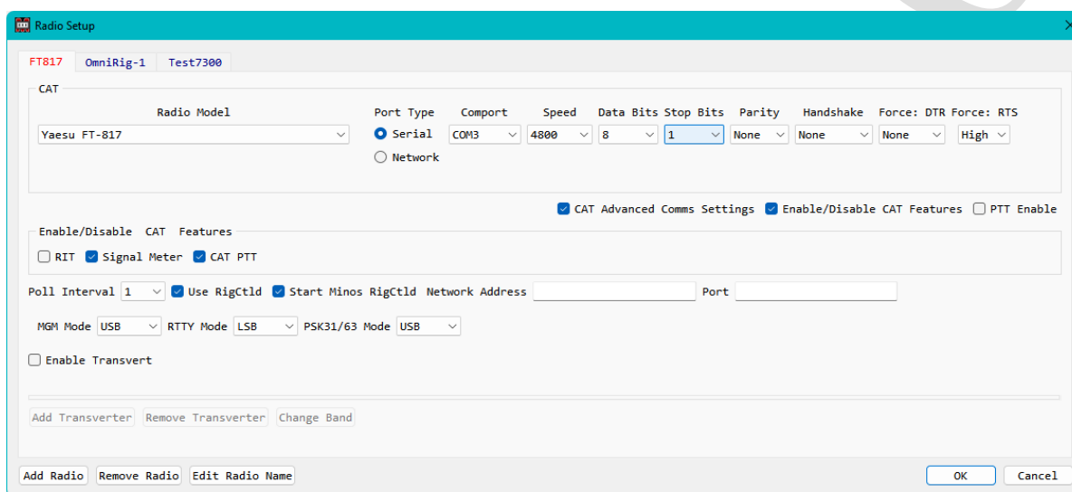
Figure 88 – Control of CAT Features
