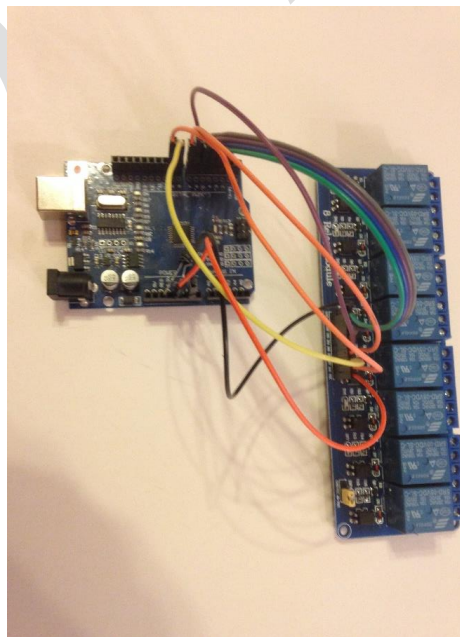
Figure 203 – Arduino and Relay Board
