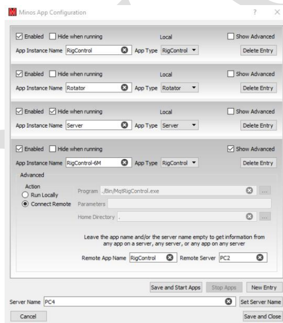
Figure 197 – Configuring two rigs, using remote RigControl
