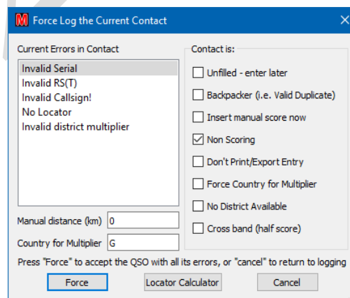
Figure 25 – Force log dialogue
