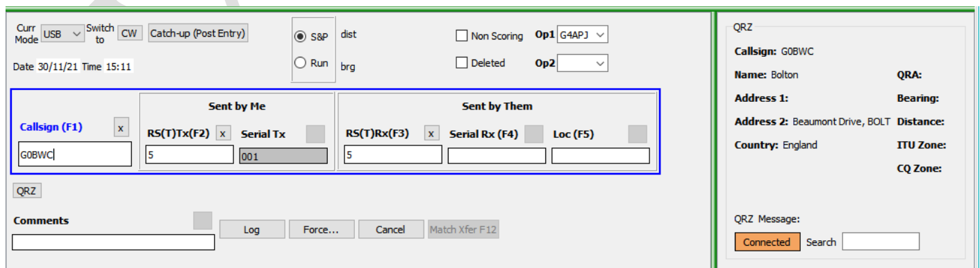
Figure 188 – QRZ lookup in the QSO panel
