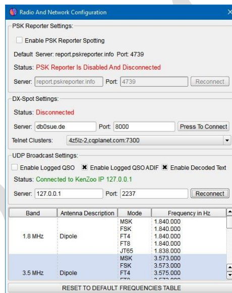
Figure 71 – MSHV configuration
