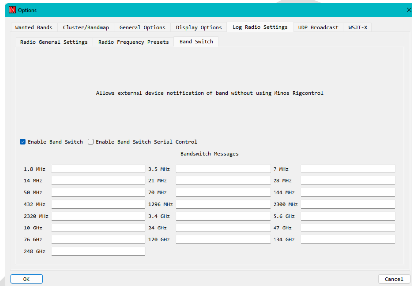
Figure 112 – Bandswitch Messages
