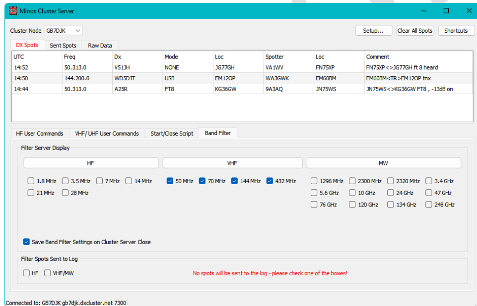
Figure 157 – Initial Cluster Server panel display
