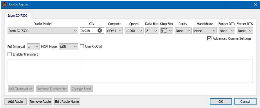
Figure 71 – Configuration of an ICOM rig
