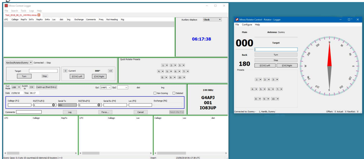
Figure 97 – Rotator connected to Logger
