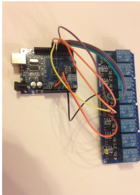
Figure 131 – Arduino and Relay Board
