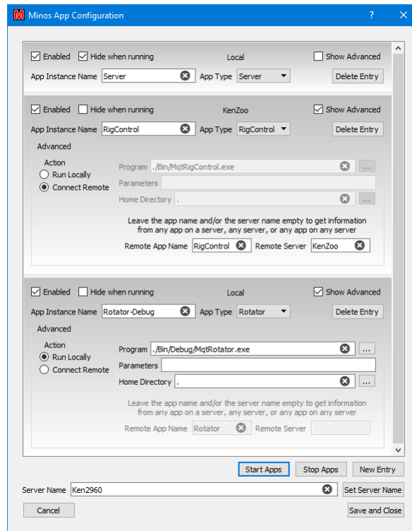
Figure 102 – Advanced configuration
