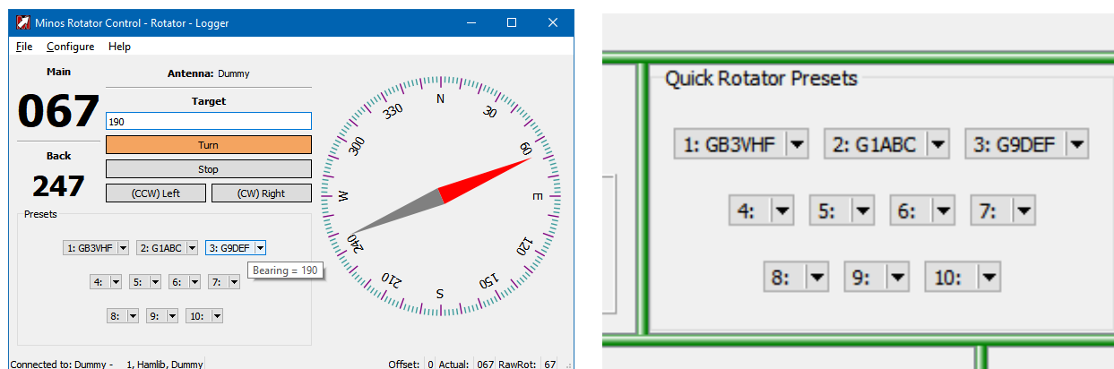
Figure 80 – Configuring pre-sets
