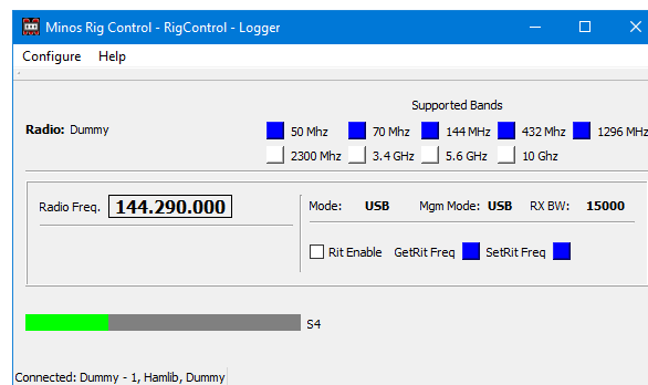
Figure 62 – RigControl operational
