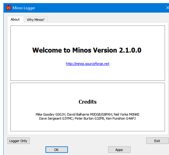
Figure 8 – Welcome screen
