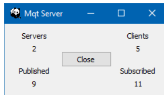
Figure 53 – Server statistics
