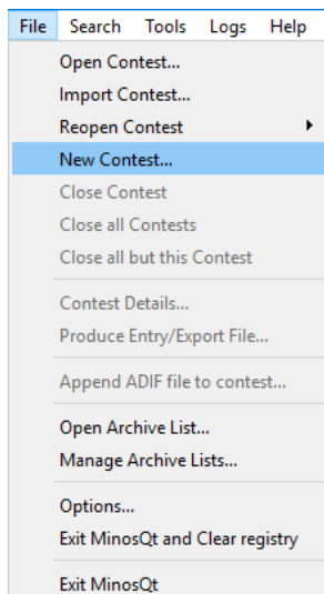
Figure 9 – File options
