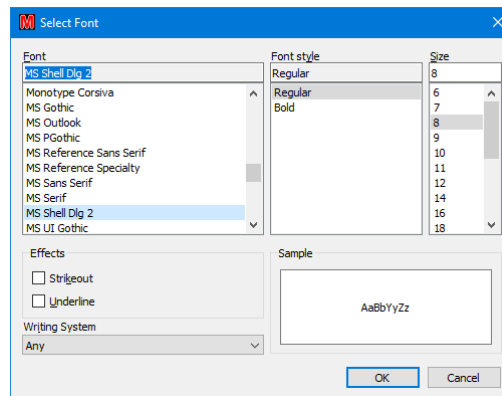
Figure 50 – Font selection
