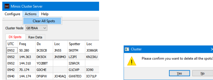
Figure 98 – Clearing spots.
