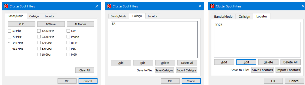
Figure 100 – Filter tabs
