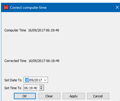
Figure 42 – Clock adjustment
