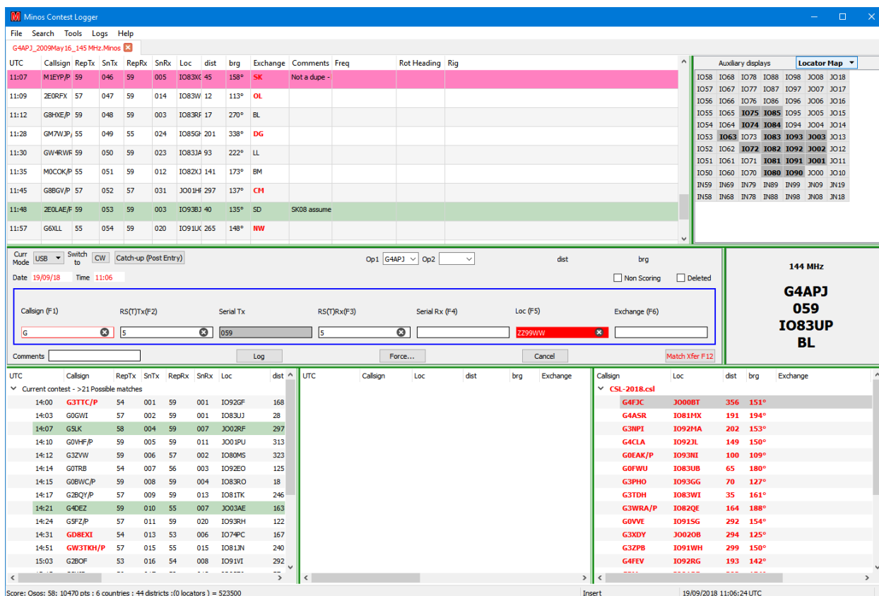
Figure 17 – Colour coding
