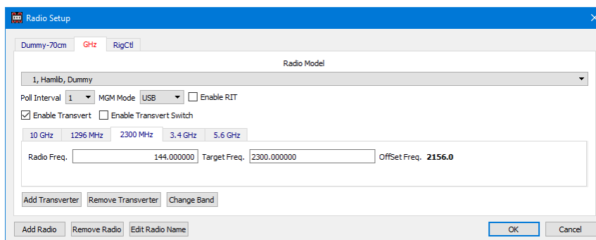
Figure 70 – Transverter definition
