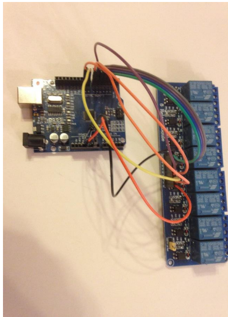
Figure 129 – Arduino and Relay Board
