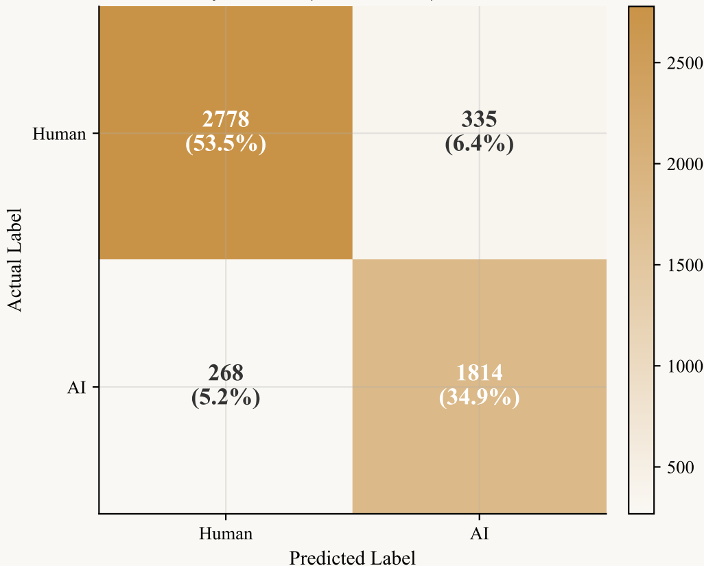
Confusion Matrix — LightGBM Accuracy: 88.4% | F1: 0.858 | AUC: 0.9549
