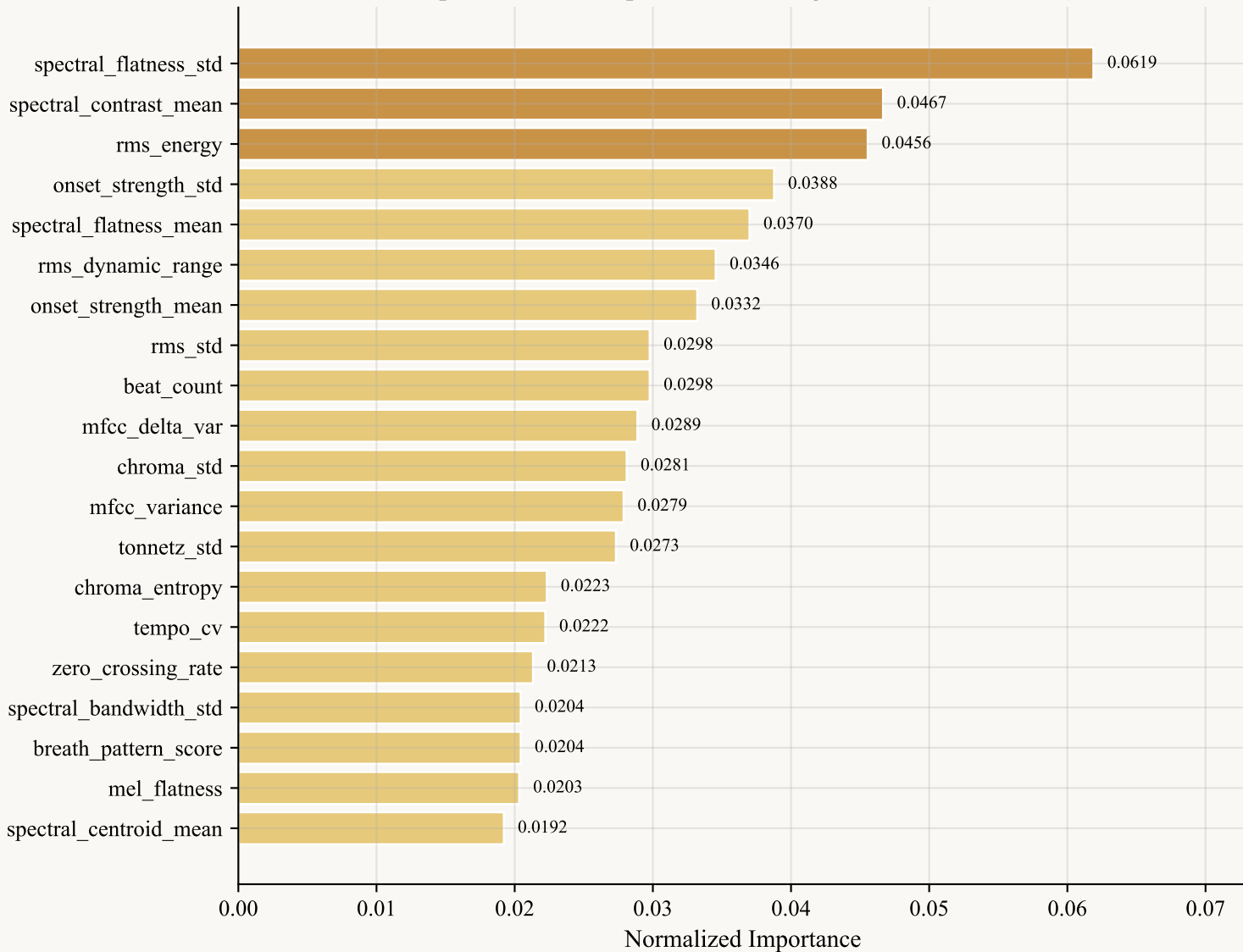
Top 20 Feature Importances — LightGBM (Best Model)
