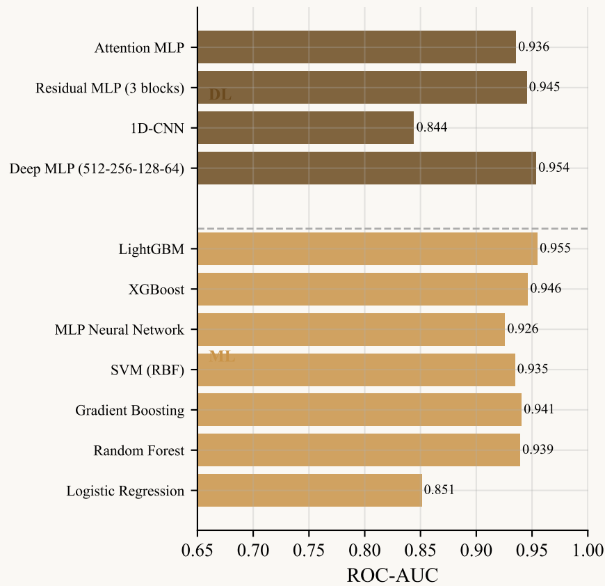
ML vs DL Model Comparison — 47 Features, 5,195 Samples, 5-Fold CV
