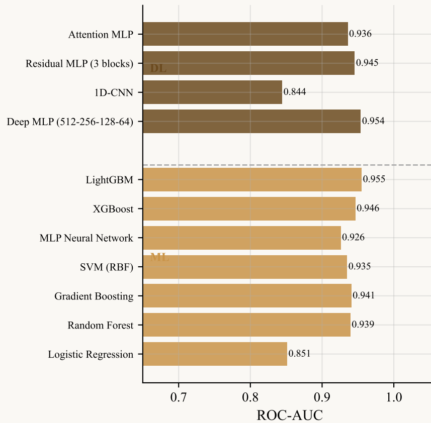
ML vs DL Model Comparison — 47 Features, 5,195 Samples, 5-Fold CV
