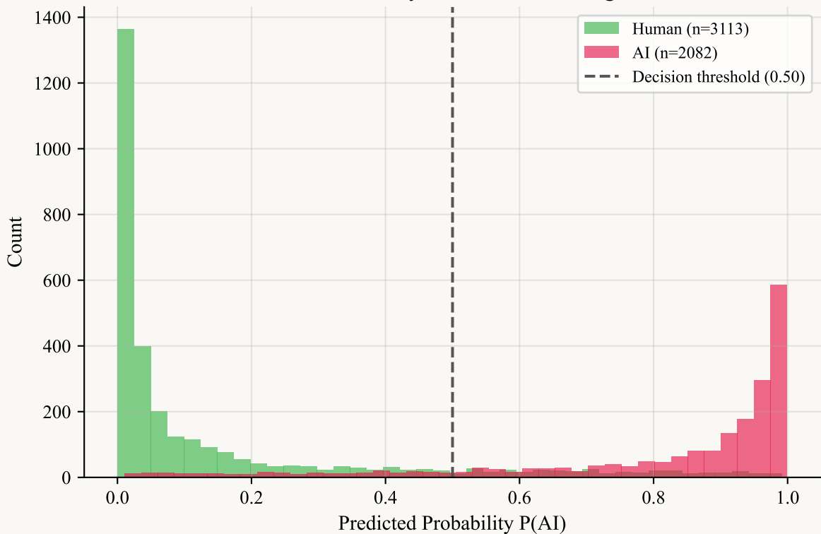
Predicted Probability Distribution — LightGBM
