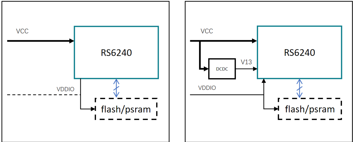
Figure 6-1 BOM Optimized (Left) and Power Optimized (Right) Mode
