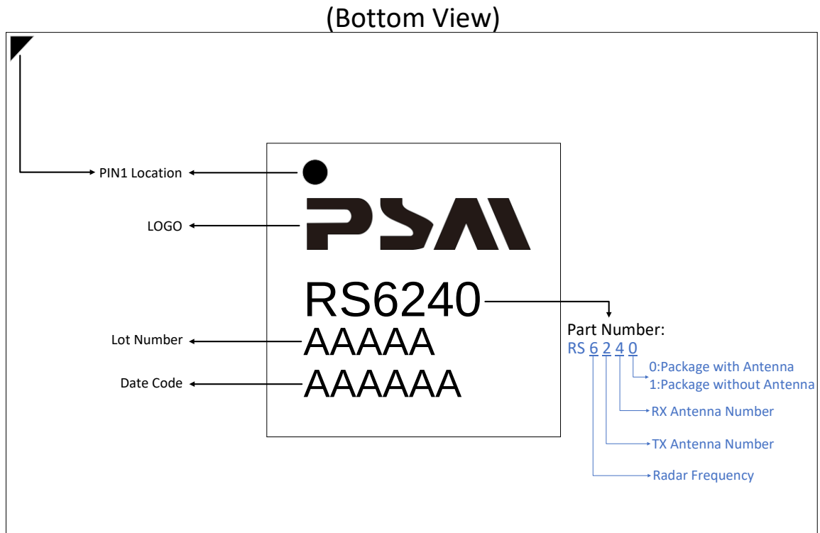
Figure 10-1 Silkscreen
