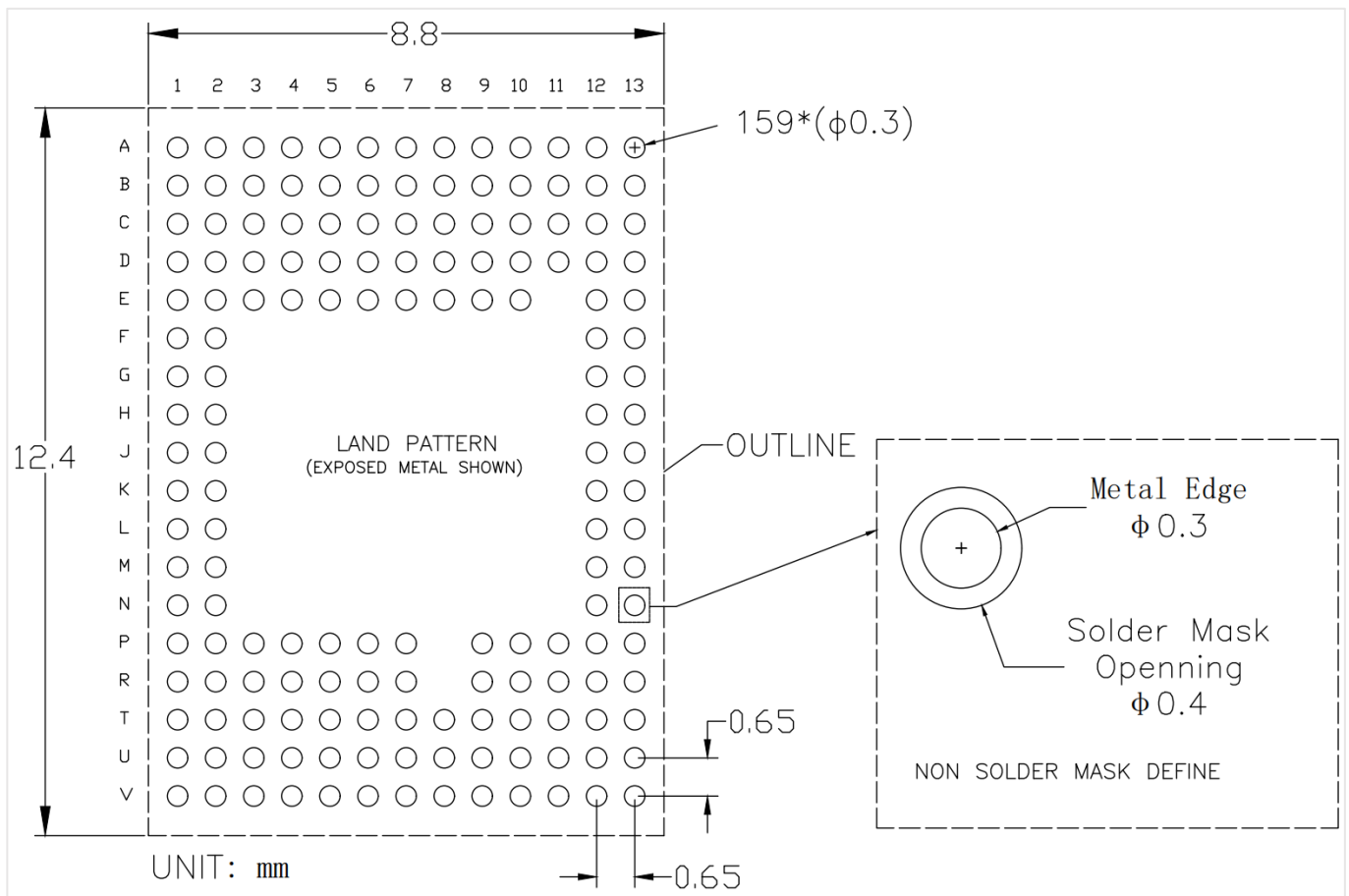
Figure 8-2 PCB Land Pattern Diagram
