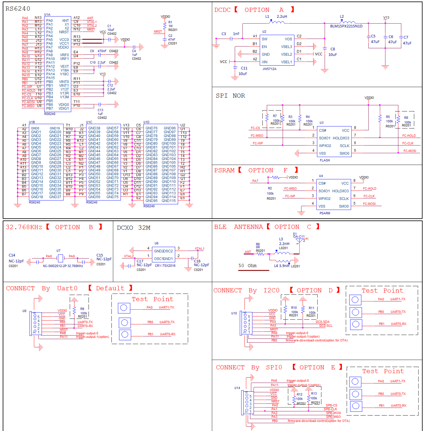
Figure 9-1 Reference Schematic
