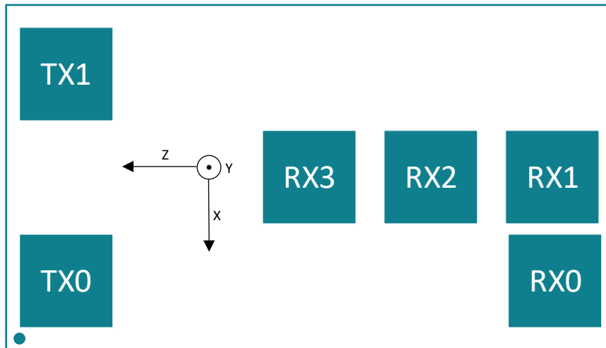
Figure 1 Antenna Configuration (Top View)
