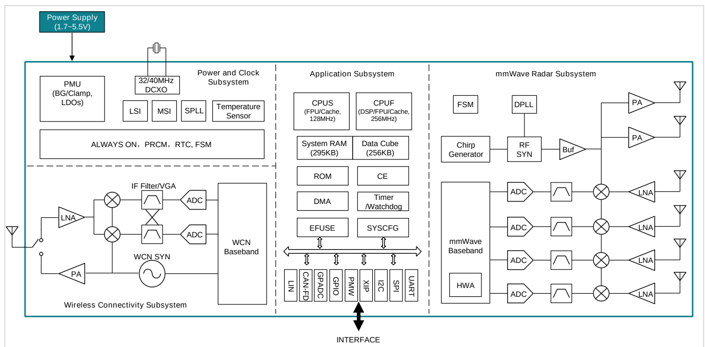
Figure 7-1 System Block Diagram
