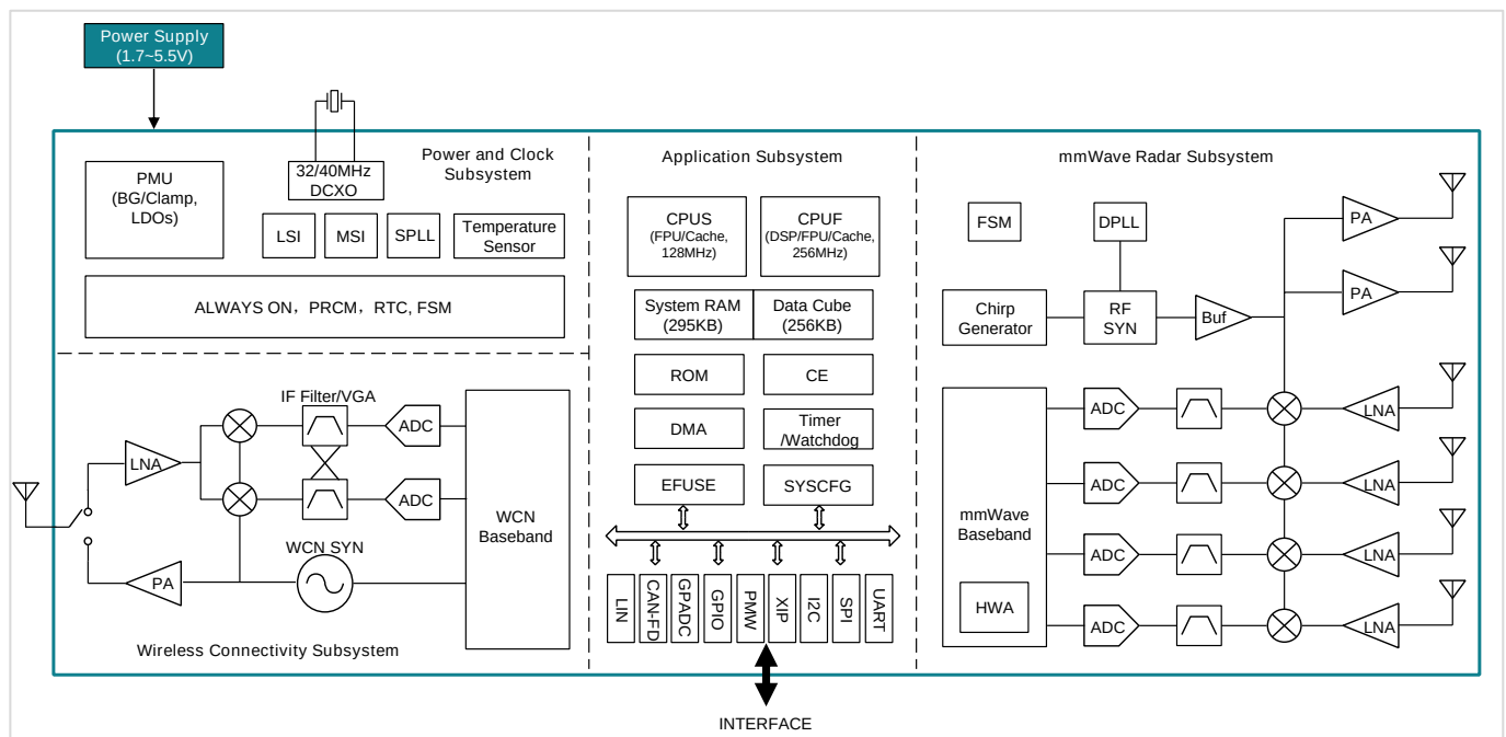
Figure 3-1 Block Diagram
