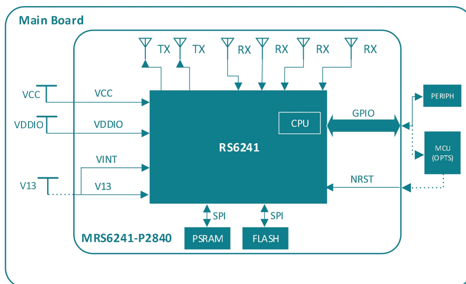
Figure 2-1 MRS6241-P2840-M81 System Application Block Diagram
