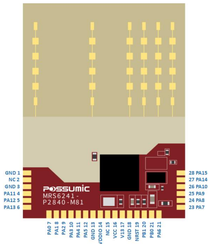
Figure 3-1 Pin Layout
