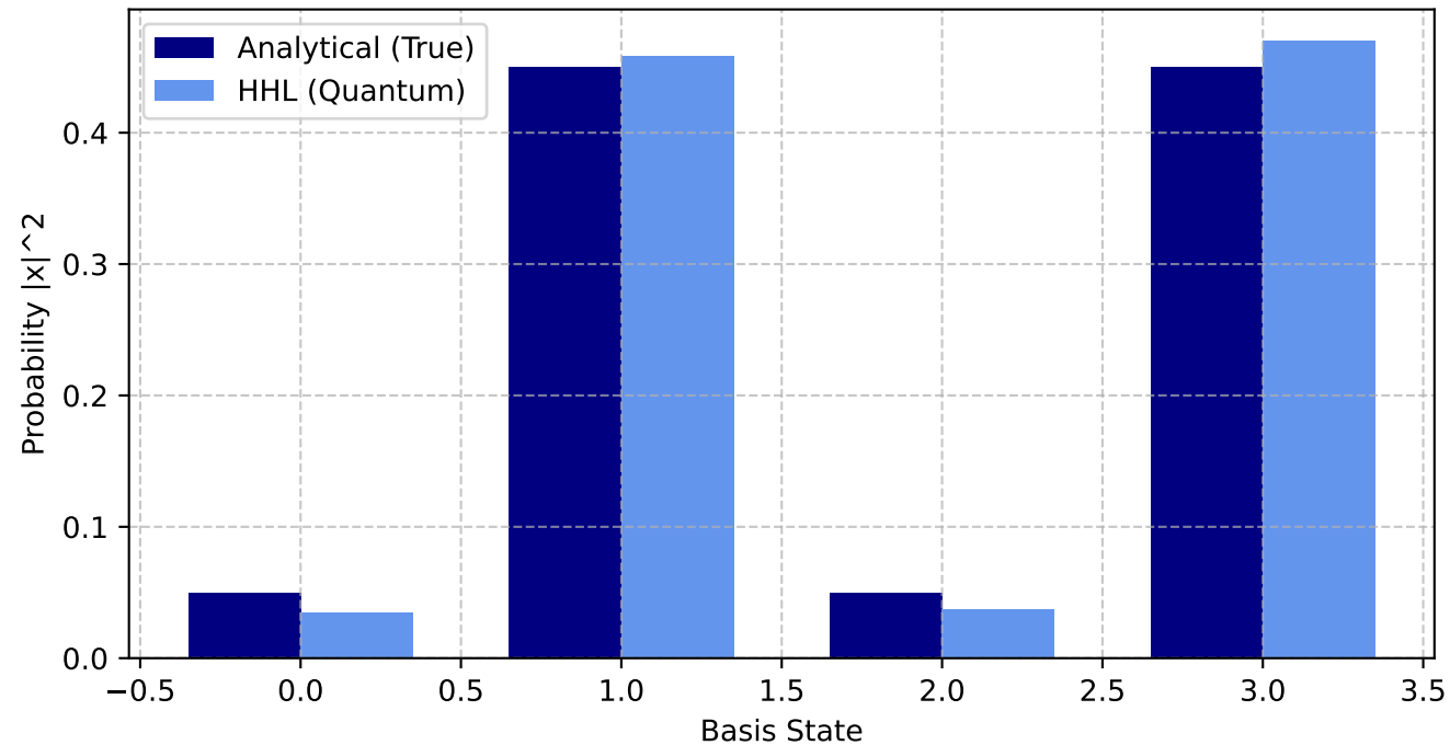
4x4 Block Diagonal
