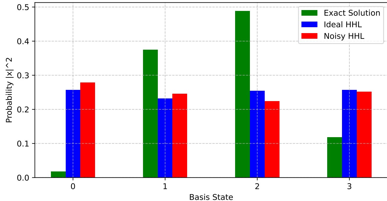
4x4 Random Dense
