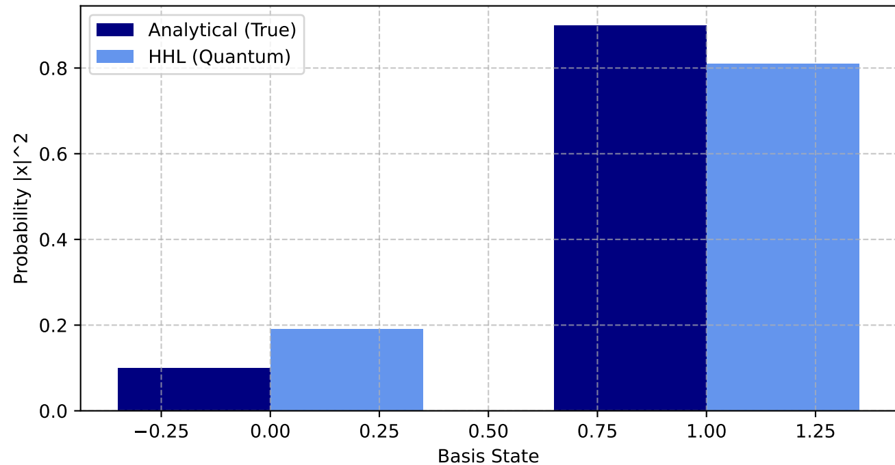
2x2 Fractional Eigenvalues
