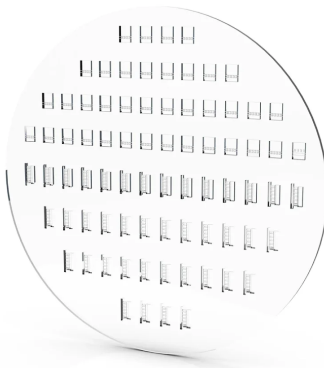
Figure 1.6: Wafer-scale fabrication of Laser-Written Vapor Cells. Multiple LWVC devices inscribed simultaneously in a single fused-silica substrate by QSENSATO Srl, demonstrating the batch-production capability of the FLICE platform. All subsequent etching, filling, and bonding steps can be performed at the wafer level. Image courtesy of QSENSATO Srl [17].
