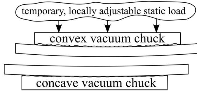
Figure 3.11: Pressure plate geometry described by Birckigt et al. [83]. The curved profiles guide contact front propagation outward from the center, reducing the probability of interface void formation.
