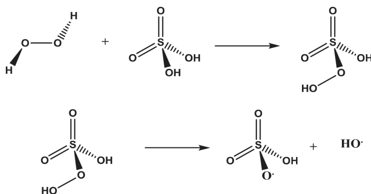
Figure 3.3: Hydroxyl radicals formation upon the decomposition of Caro's acid in Piranha solution. From [62].
