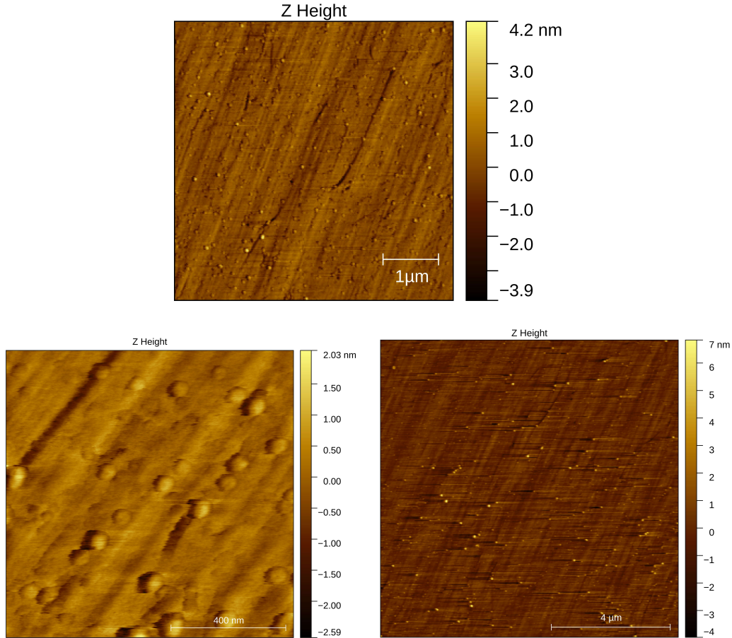
Figure 6: 2D Surface images obtained through AFM
