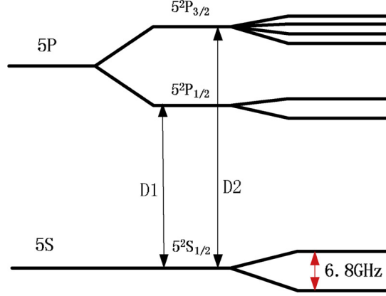
Figure 8: Energy level diagram showing the D1 and D2 transitions in an alkali metal atom. From [21]
