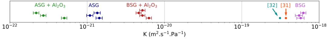
Figure 9: Comparison of the permeability constant K across uncoated borofloat, uncoated aluminosilicate, \text{Al}_2\text{O}_3 -coated borofloat, and \text{Al}_2\text{O}_3 -coated aluminosilicate glasses. From [26].
