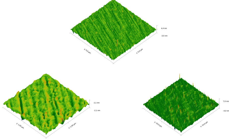
Figure 7: 3D Surface images obtained through AFM
