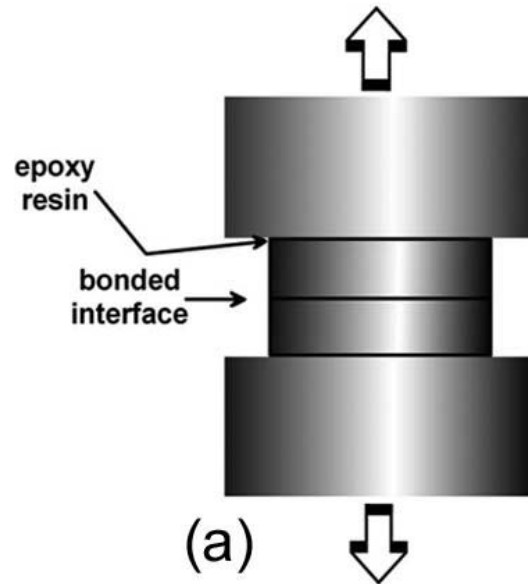
Figure 4.3: Schematic diagram of the tensile test setup for bonding strength measurement. The bonded wafer pair is glued to metal fixtures and subjected to perpendicular tensile force. Adapted from [10].
