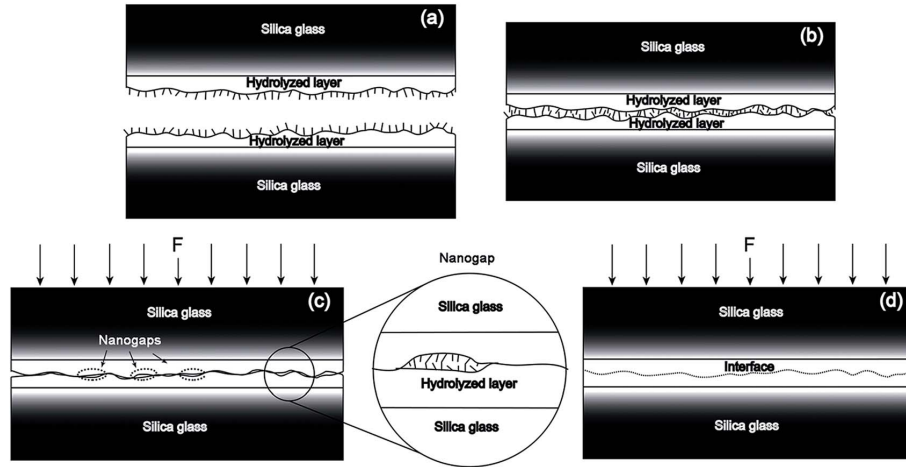
Figure 3.6: Effect of applied pressure on the bonding process. Forces perpendicular to the interface suppress void formation by closing residual gaps between surface asperities. From [39].
