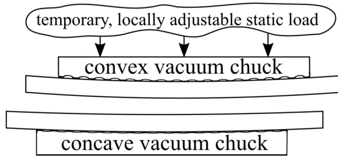
Figure 3.7: Pressure plate geometry described by Birckigt et al. [42]. The curved profiles guide contact front propagation outward from the center, reducing the probability of interface void formation.
