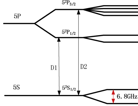
Figure 11: Energy level diagram showing the D1 and D2 transitions in an alkali metal atom. From [25]
