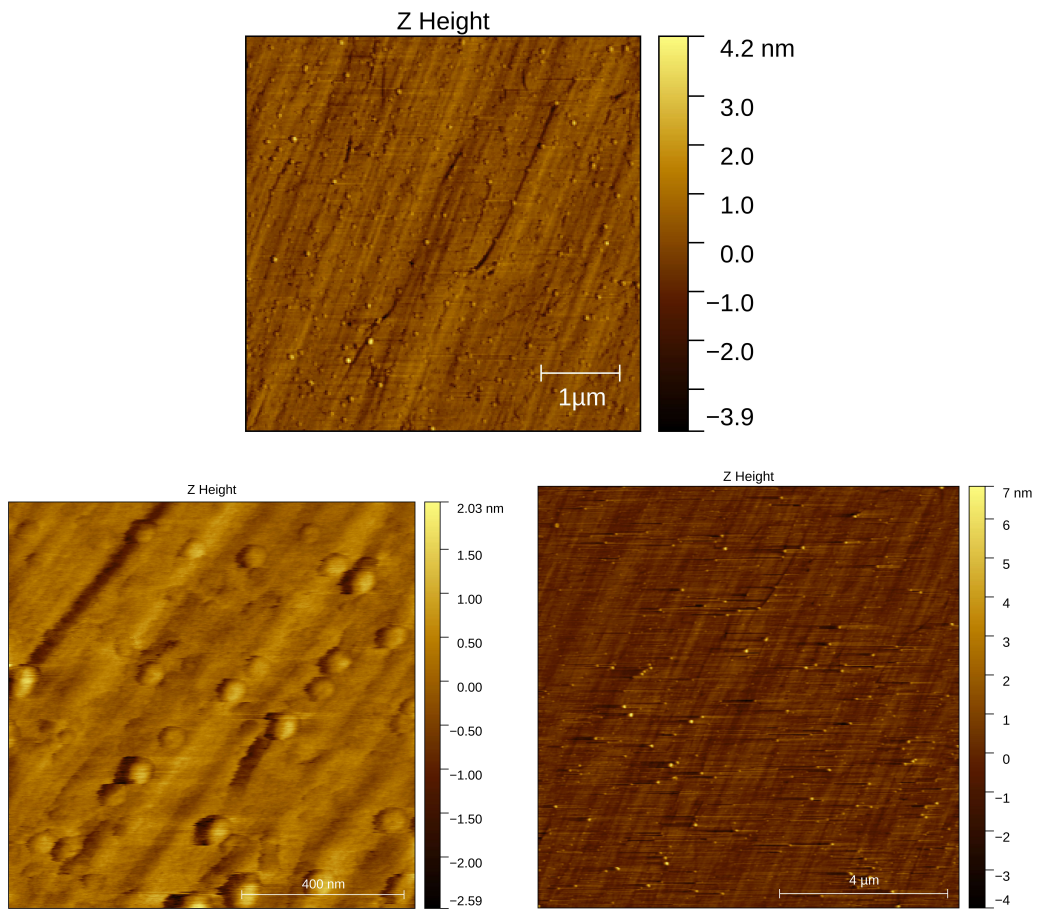
Figure 8: 2D Surface images obtained through AFM in three different parts of the pristine Nanoquartz disk's surface.
