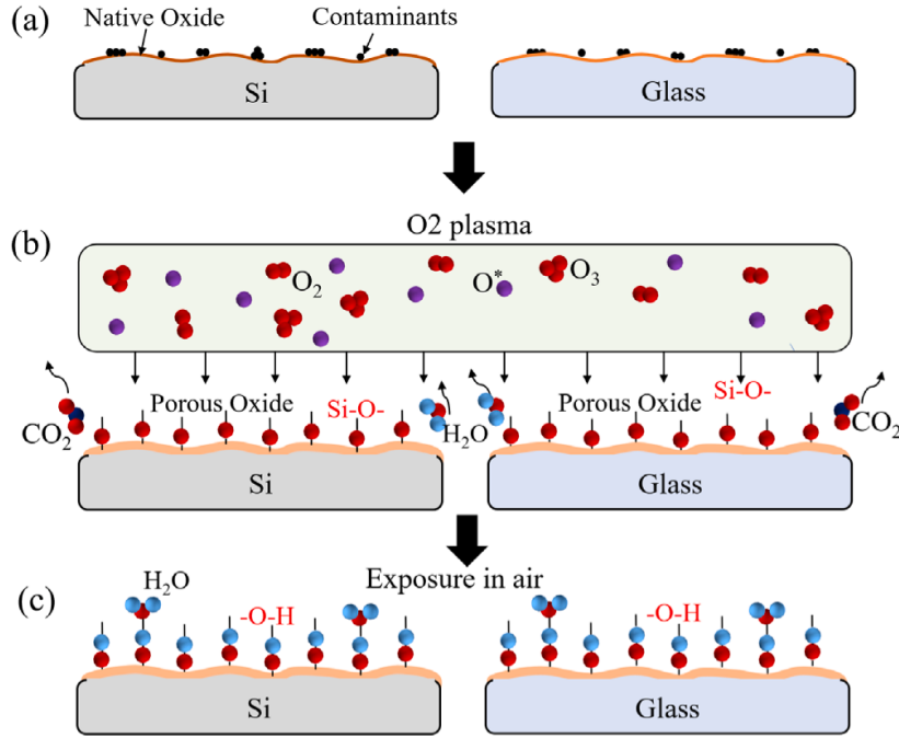
Figure 2: Effects of plasma treatment on silica surfaces. Plasma helps to remove contaminants while increasing the number of available silanol groups. Adapted from [4]
