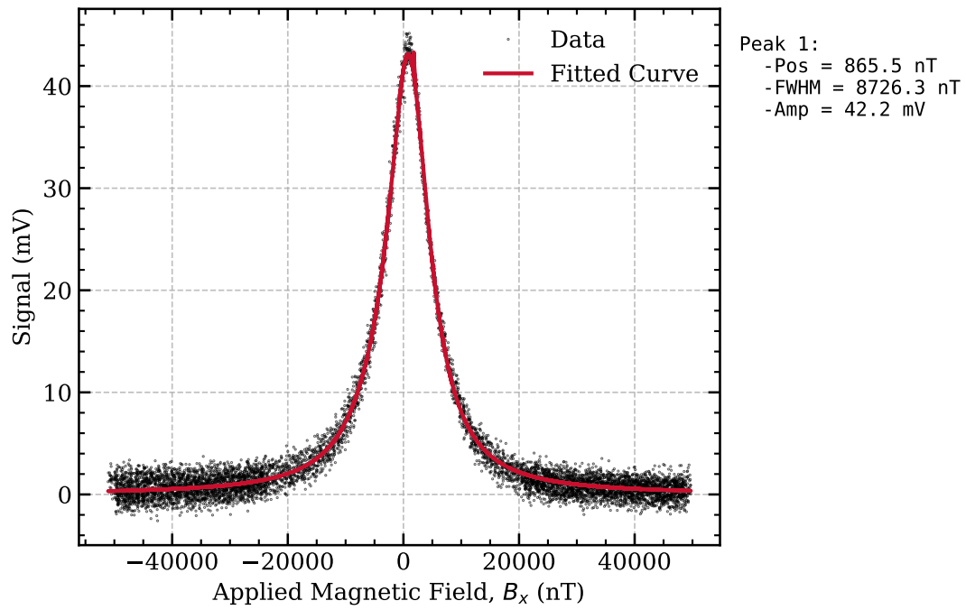
Figure 14: Raw data and Lorentzian fit of the Hanle resonance obtained for the optimal DC field configuration ( B_y = 0 nT, B_z = 4815 nT)
