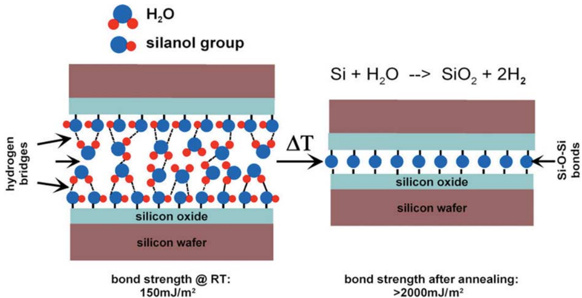
Figure 3.3: Bonding process of two fused silica surfaces. Silanol ( \text{Si-OH} ) groups initially form hydrogen bonds across the interface; subsequent thermal treatment converts these into permanent covalent \text{Si-O-Si} bonds. From [10].
