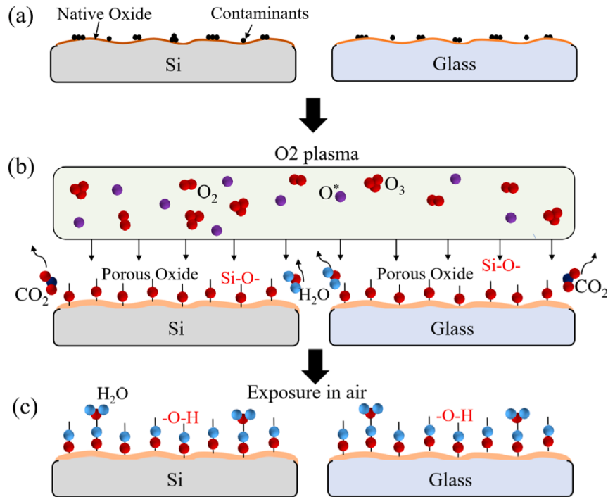
Figure 3.4: Effects of plasma treatment on silica surfaces. Plasma removes contaminants and increases the density of available silanol groups. Adapted from [42].
