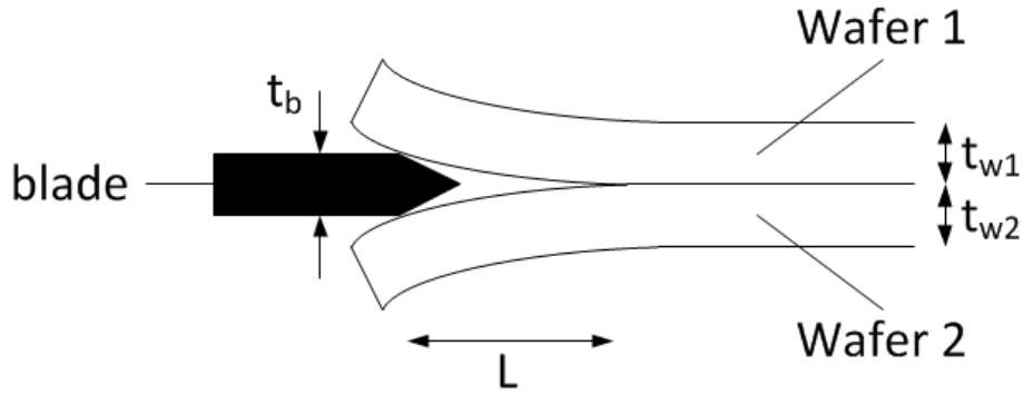
Figure 4.6: Illustration of the razor blade method. A razor blade is inserted between the bonded surfaces in order to quantify the bonding energy between them. From [56].
