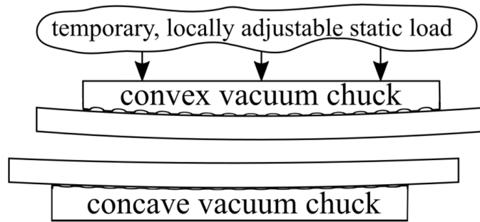
Figure 3.7: Pressure plate geometry described by Birckigt et al. [50]. The curved profiles guide contact front propagation outward from the center, reducing the probability of interface void formation.
