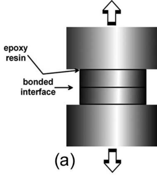
Figure 4.8: Schematic diagram of the tensile test setup for bonding strength measurement. The bonded wafer pair is glued to metal fixtures and subjected to perpendicular tensile force. Adapted from [10].
