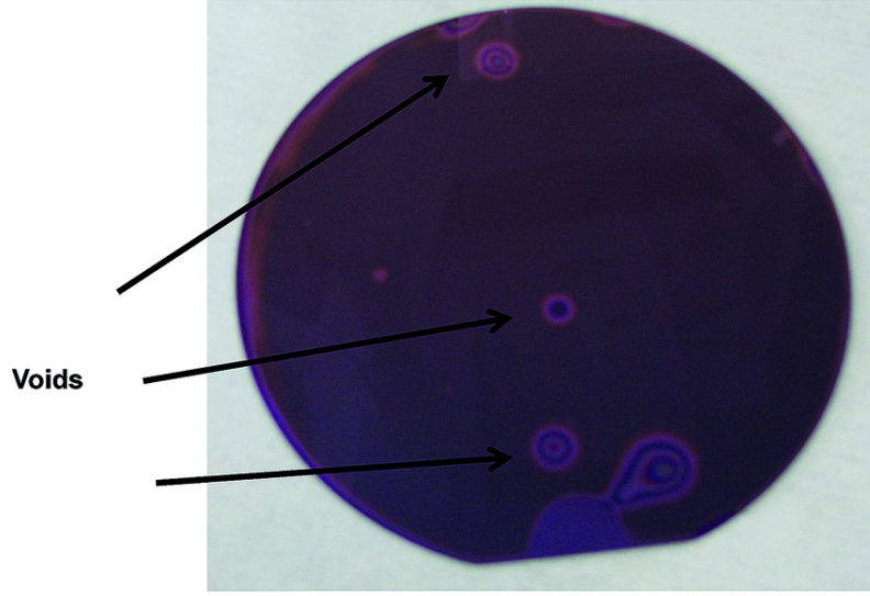
Figure 4.5: Newton rings being formed on the interfase of a SiN-glass wafer. From [54].
