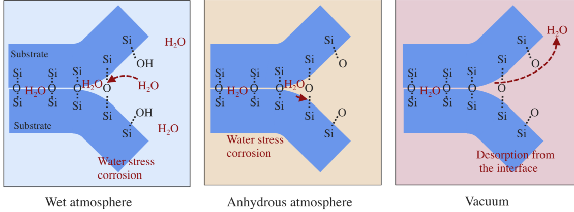
Figure 4.7: Schematic representation of water stress corrosion at the hydrophilic bonding interface during debonding under controlled atmospheres. Left: wet atmosphere showing ambient water attack on Si–O–Si bonds. Center: anhydrous (dry) atmosphere with reduced water availability. Right: vacuum conditions with partial desorption of interfacial water. Adapted from [55].
