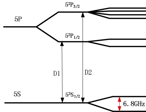
Figure 4.9: Energy level diagram showing the D1 and D2 transitions in an alkali metal atom. From [66]
