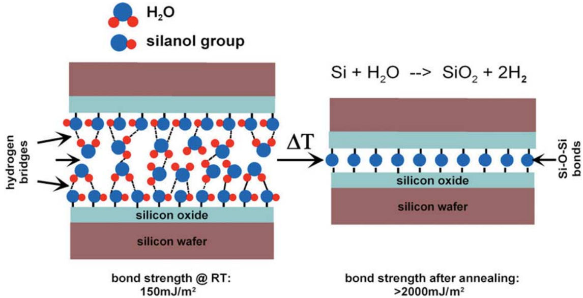
Figure 3.1: Bonding process of two Fused Silica surfaces. Initially, hydrogen bonds are formed between them due to the presence of Silanol (Si-OH) groups. These bonds are subsequently transformed into stronger covalent bonds through thermal treatment. From [7].
