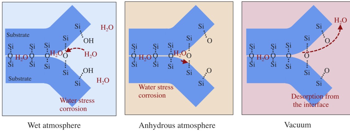
Figure 4.2: Schematic representation of water stress corrosion at the hydrophilic bonding interface during debonding under controlled atmospheres. Left: wet atmosphere showing ambient water attack on Si–O–Si bonds. Center: anhydrous (dry) atmosphere with reduced water availability. Right: vacuum conditions with partial desorption of interfacial water. Adapted from [42].
