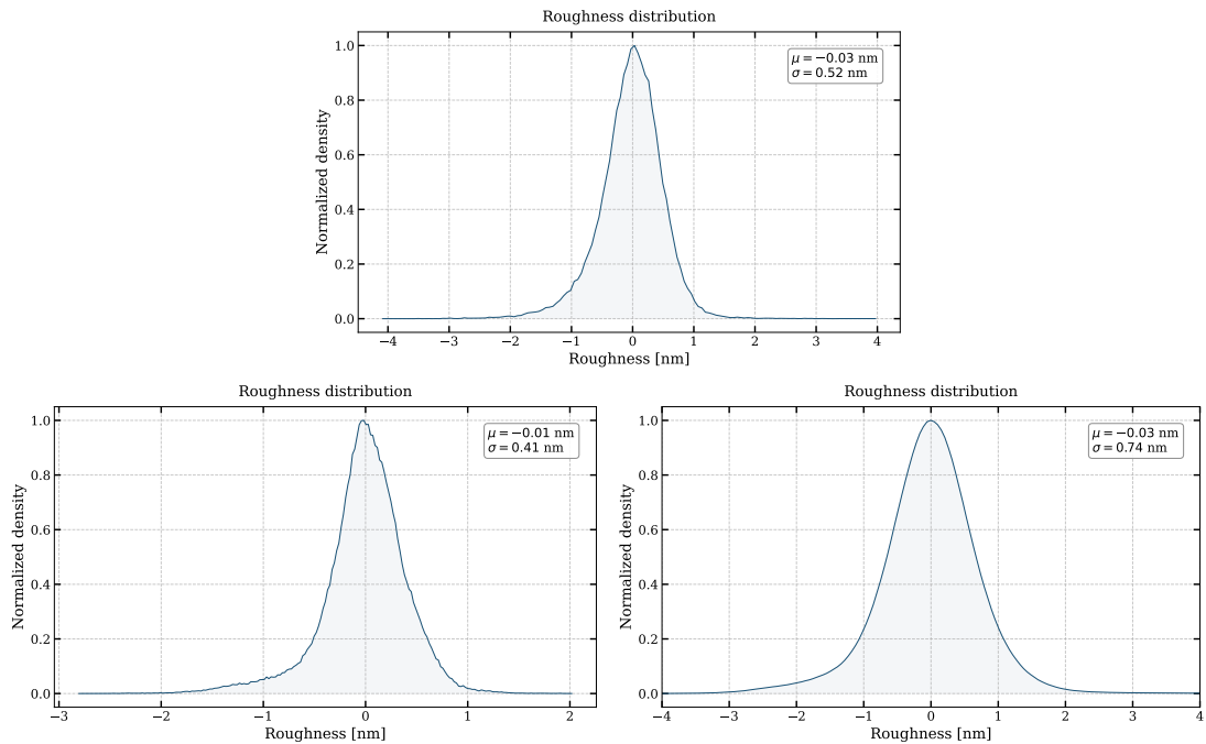
Figura 4.7: Surface roughness distribution obtained through AFM. It can be seen that most of the defects are below the 1 nm range. Furthermore, the mean ( \mu ) is close to zero, confirming that the surface is uniform.
