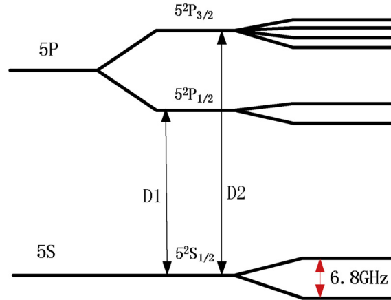
Figura 4.8: Energy level diagram showing the D1 and D2 transitions in an alkali metal atom. From [54]
