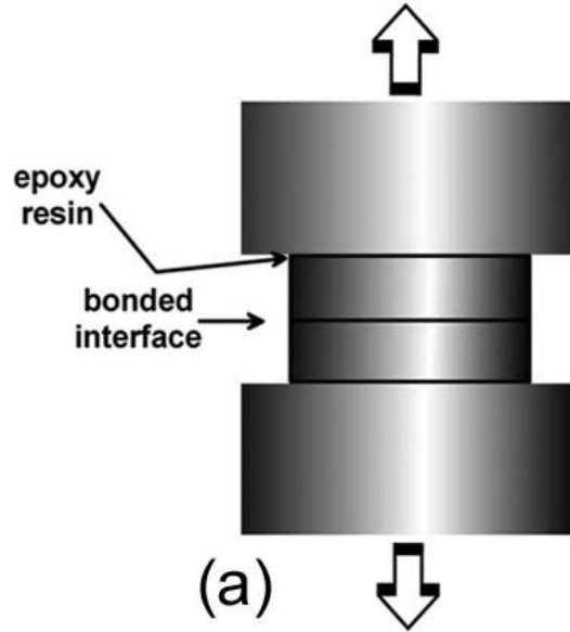
Figure 4.3: Schematic diagram of the tensile test setup for bonding strength measurement. The bonded wafer pair is glued to metal fixtures and subjected to perpendicular tensile force. Adapted from [7].
