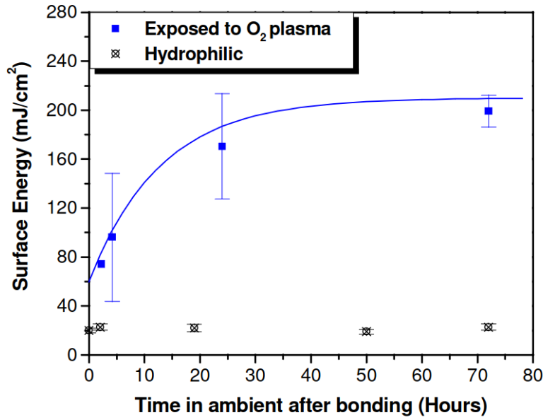
Figura 3.3: Bonding energy evolution with time. From [32]
