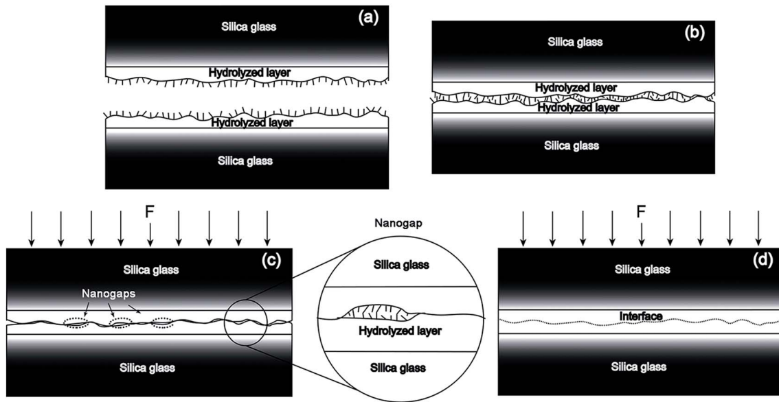
Figure 3.4: Effects of pressure in the bonding process. Interface voids can be prevented by applying forces in the direction perpendicular to the interface. From [36]
