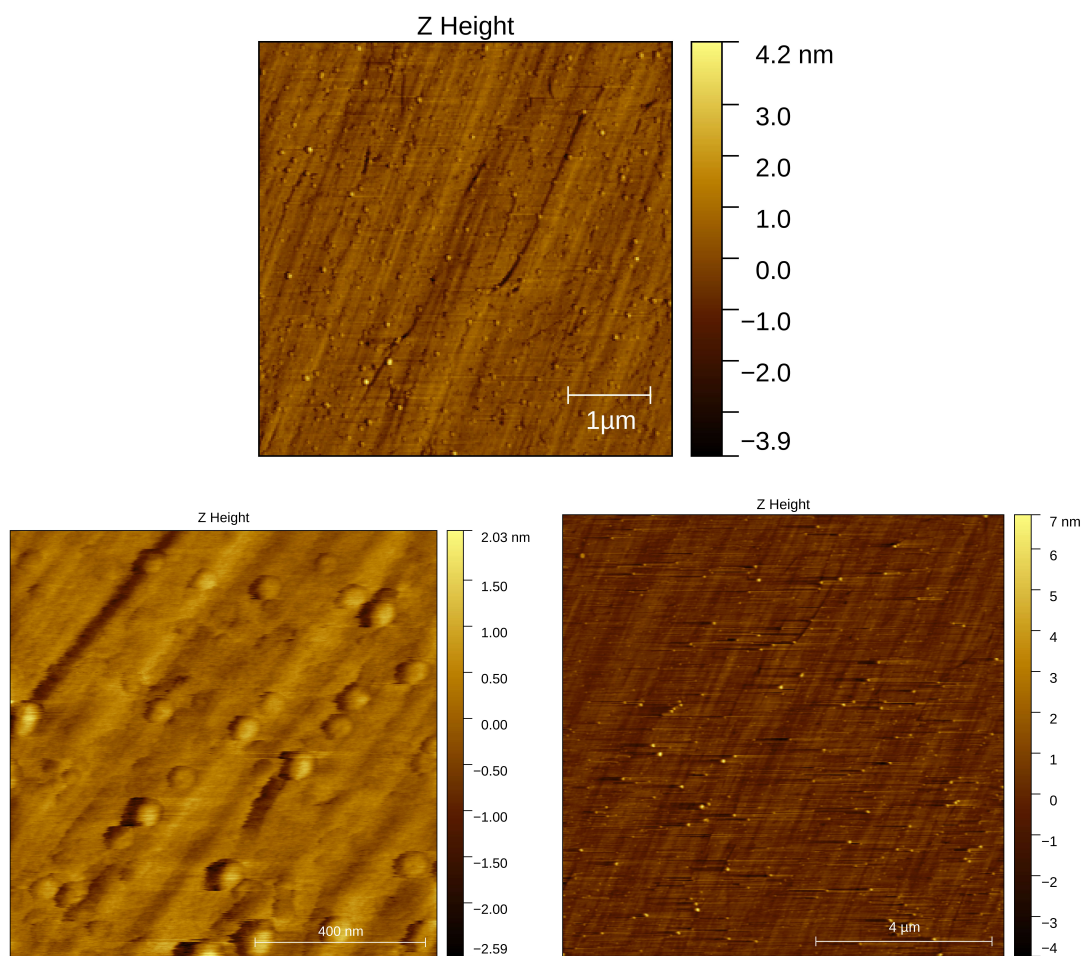
Figura 4.5: 2D Surface images obtained through AFM in three different parts of the pristine Nanoquartz disk's surface.
