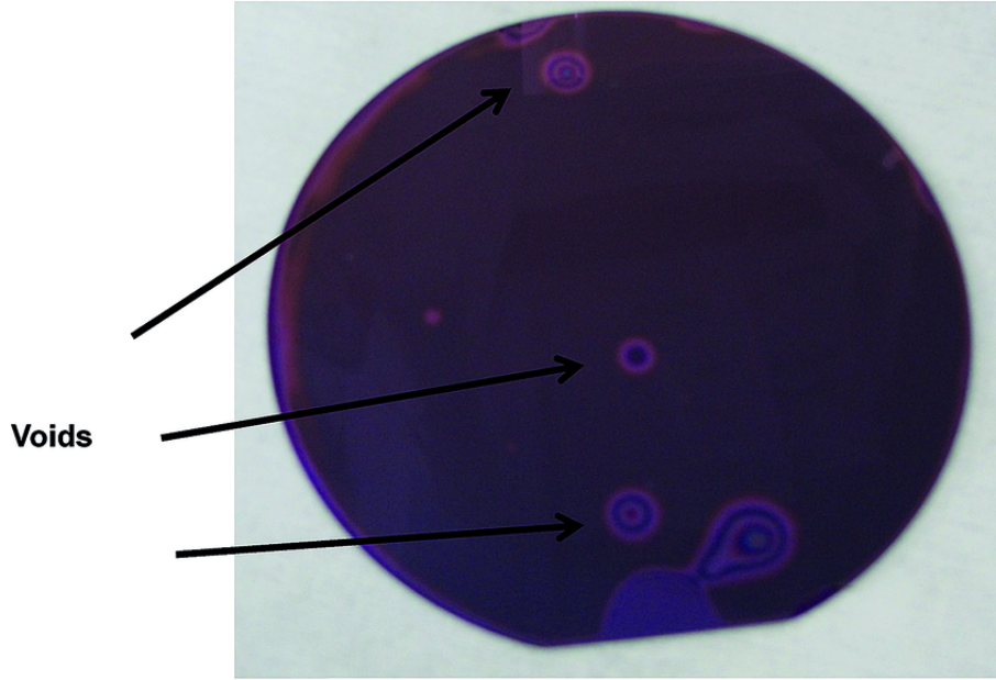
Figura 4.1: Newton rings being formed on the interphase of a SiN-glass wafer. From [41].
