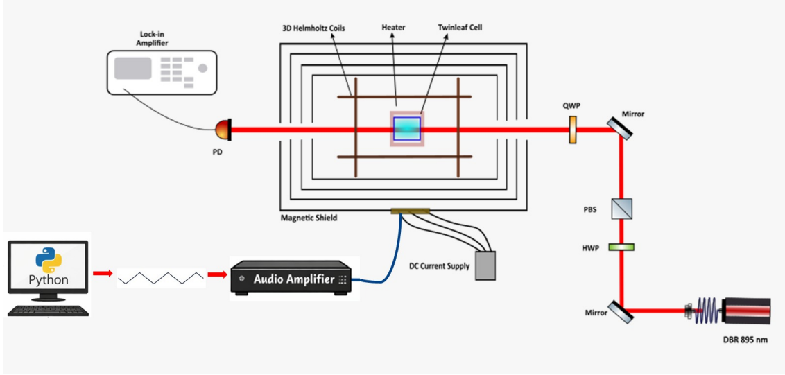
Figura 5.1: Experimental setup used to detect Hanle resonance
