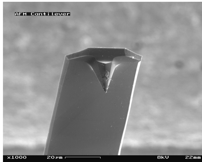
Figura 4.4: View of cantilever in Atomic Force Microscope (magnification 1000x) [48]
