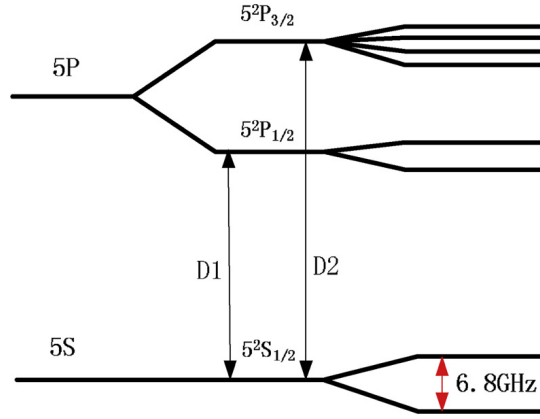
Figure 14: Energy level diagram showing the D1 and D2 transitions in an alkali metal atom. From [39]
