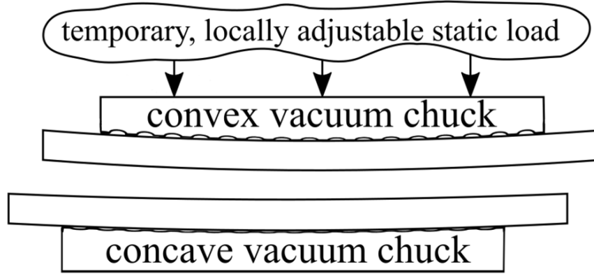
Figure 5: Setup described by Birckigt et al. [22]
