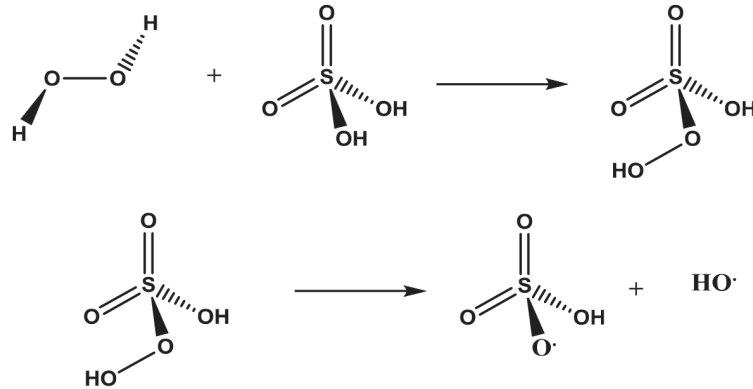
Figure 3.3: Hydroxyl radicals formation upon the decomposition of Caro's acid in Piranha solution. From [44].
