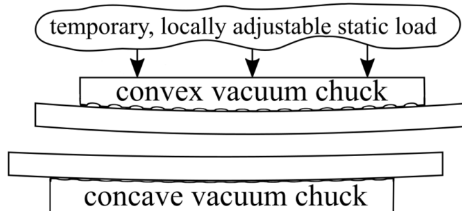
Figure 3.11: Pressure plate geometry described by Birckigt et al. [65]. The curved profiles guide contact front propagation outward from the center, reducing the probability of interface void formation.
