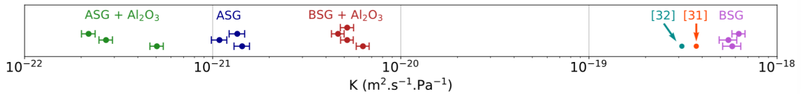
Figure 3.8: Comparison of the permeability constant K across uncoated borofloat, uncoated aluminosilicate, \text{Al}_2\text{O}_3 -coated borofloat, and \text{Al}_2\text{O}_3 -coated aluminosilicate glasses. From [34].
