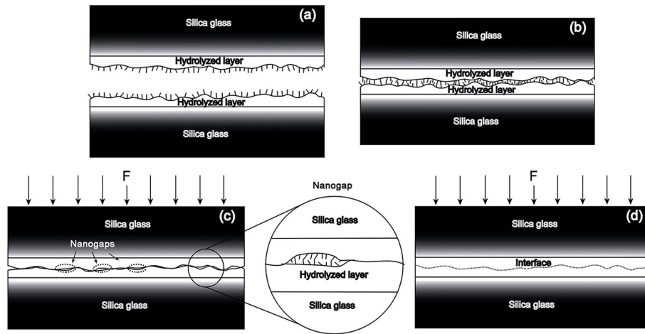
Figure 3.6: Effect of applied pressure on the bonding process. Forces perpendicular to the interface suppress void formation by closing residual gaps between surface asperities. From [43].
