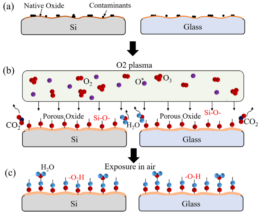
Figure 3.4: Effects of plasma treatment on silica surfaces. Plasma removes contaminants and increases the density of available silanol groups. Adapted from [46].
