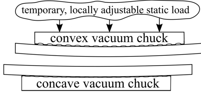
Figure 3.7: Pressure plate geometry described by Birckigt et al. [55]. The curved profiles guide contact front propagation outward from the center, reducing the probability of interface void formation.
