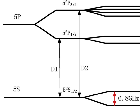
Figure 4.11: Energy level diagram showing the D1 and D2 transitions in an alkali metal atom. From [76]
