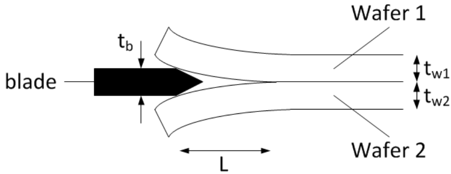
Figure 4.8: Illustration of the razor blade method. A razor blade is inserted between the bonded surfaces in order to quantify the bonding energy between them. From [66].
