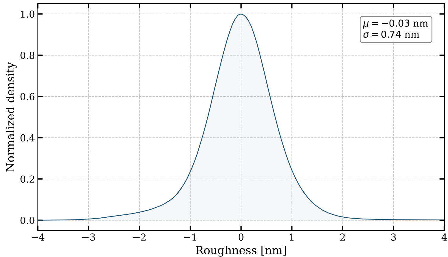
Roughness distribution
