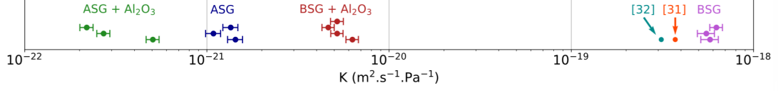
Figure 10: Comparison of the permeability constant K across uncoated borofloat, uncoated aluminosilicate, \text{Al}_2\text{O}_3 -coated borofloat, and \text{Al}_2\text{O}_3 -coated aluminosilicate glasses. From [27].
