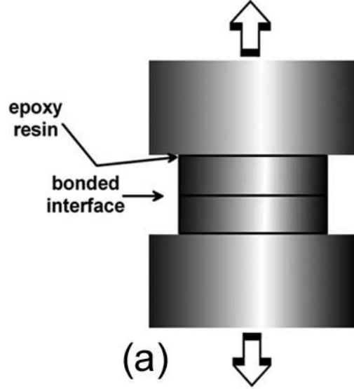
Figure 8: Schematic diagram of the tensile test setup for bonding strength measurement. The bonded wafer pair is glued to metal fixtures and subjected to perpendicular tensile force. Adapted from [23].
