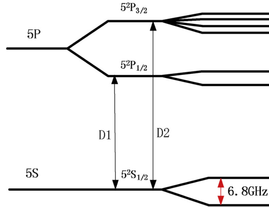
Figure 13: Energy level diagram showing the D1 and D2 transitions in an alkali metal atom. From [32]
