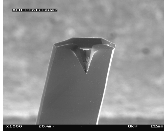
Figure 9: View of cantilever in Atomic Force Microscope (magnification 1000x) [26]
