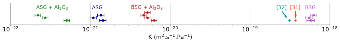
Figure 3.8: Comparison of the permeability constant K across uncoated borofloat, uncoated aluminosilicate, Al 2 O 3 -coated borofloat, and Al 2 O 3 -coated aluminosilicate glasses. From [24].
