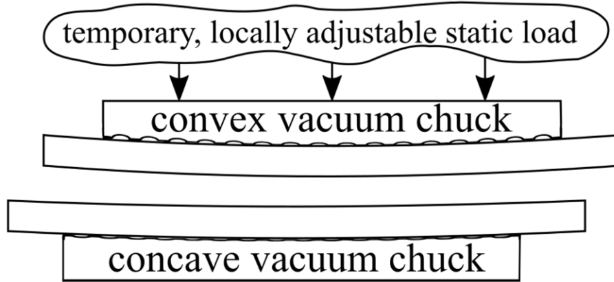
Figure 3.7: Pressure plate geometry described by Birckigt et al. [42]. The curved profiles guide contact front propagation outward from the center, reducing the probability of interface void formation.
