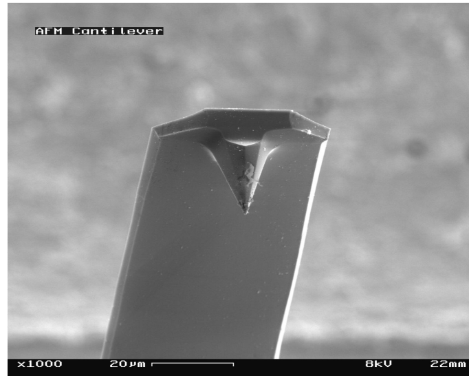
Figure 4.4: View of cantilever in Atomic Force Microscope (magnification 1000x) [59]
