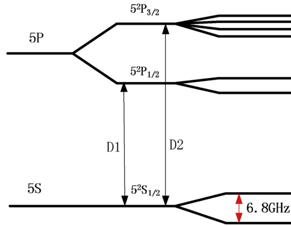
Figure 4.7: Energy level diagram showing the D1 and D2 transitions in an alkali metal atom. From [64]
