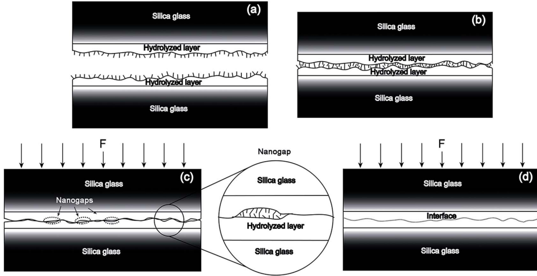
Figure 4: Effects of pressure in the bonding process. Interface voids can be prevented by applying forces in the direction perpendicular to the interface. From [27]
