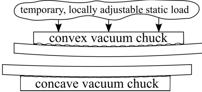
Figure 5: Setup described by Birckigt et al. [30]
