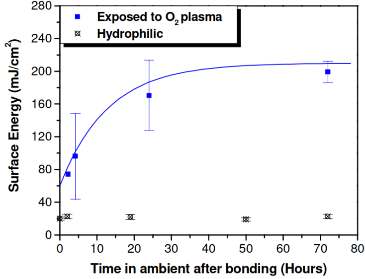
Figure 3: Bonding energy evolution with time. From [25]
