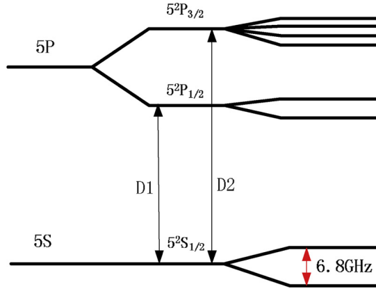
Figure 14: Energy level diagram showing the D1 and D2 transitions in an alkali metal atom. From [45]
