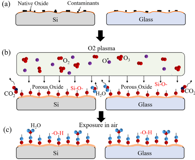
Figure 2: Effects of plasma treatment on silica surfaces. Plasma helps to remove contaminants while increasing the number of available silanol groups. Adapted from [22]
