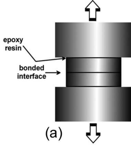
Figure 7: Schematic diagram of the tensile test setup for bonding strength measurement. The bonded wafer pair is glued to metal fixtures and subjected to perpendicular tensile force. Adapted from [21].
