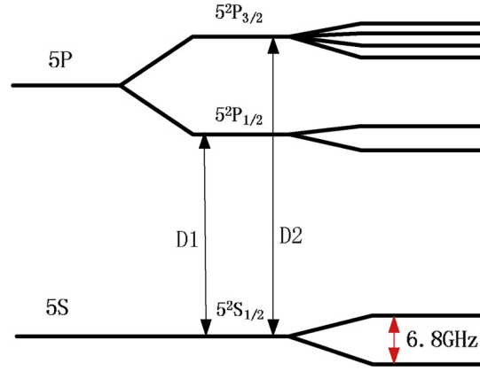
Figure 12: Energy level diagram showing the D1 and D2 transitions in an alkali metal atom. From [30]
