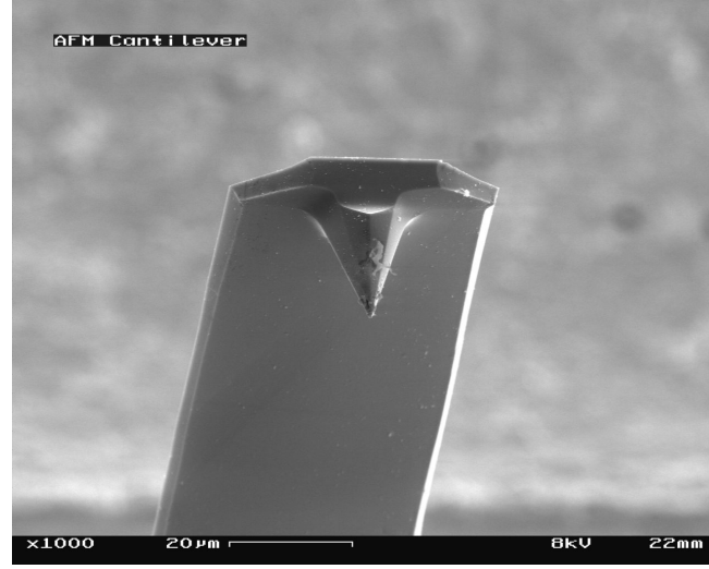
Figure 8: View of cantilever in Atomic Force Microscope (magnification 1000x) [24]
