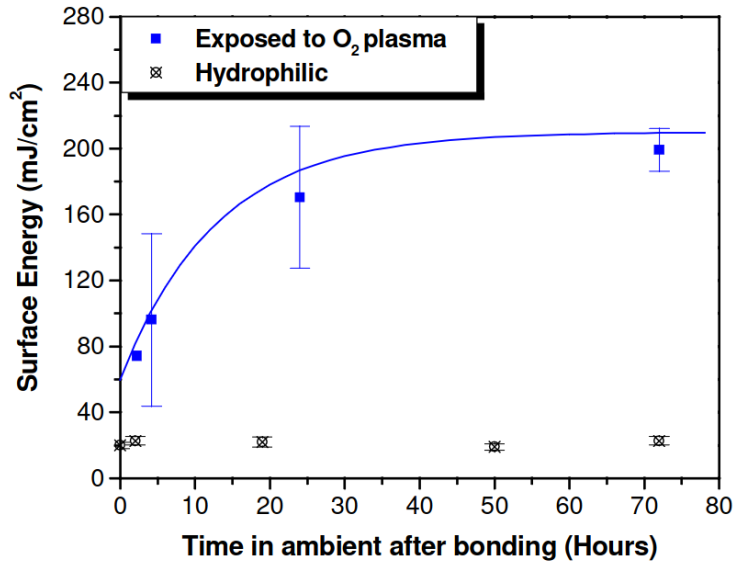
Figure 3: Bonding energy evolution with time. From [17]
