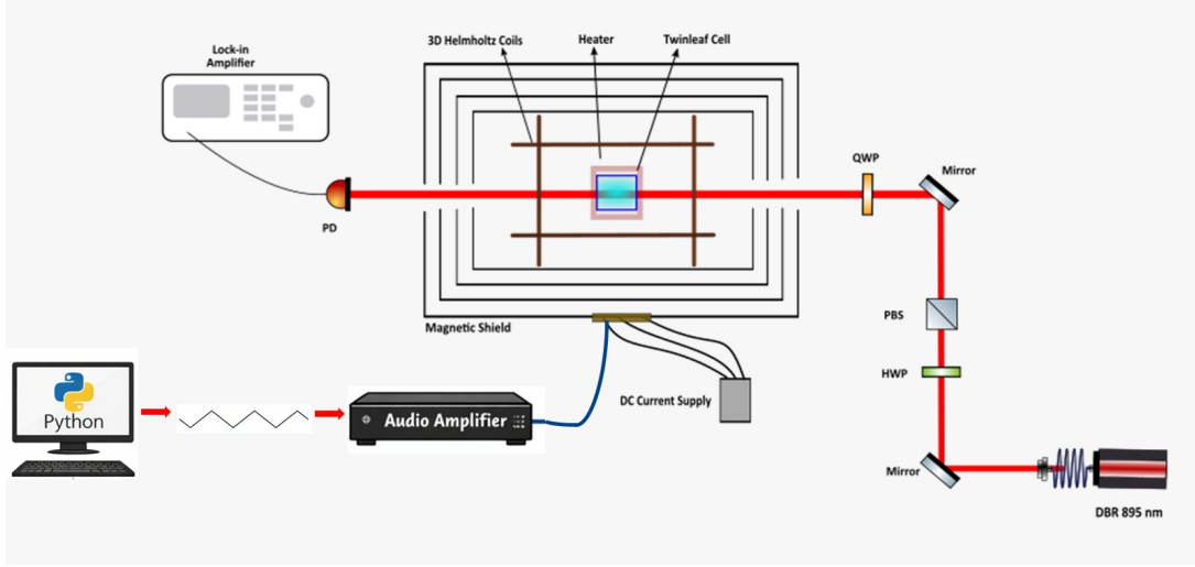
Figure 14: Experimental setup used to detect Hanle resonance
