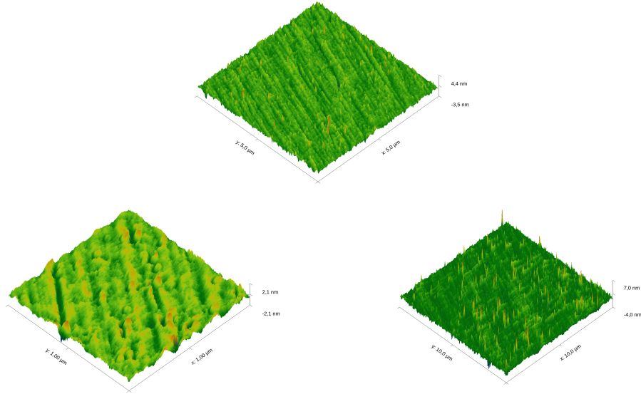
Figure 11: 3D Surface images obtained through AFM in three different parts of the pristine Nanoquartz disk's surface.
