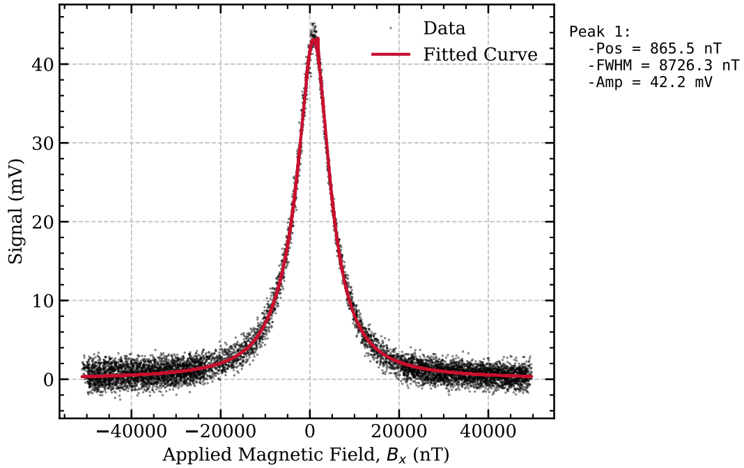
Figure 16: Raw data and Lorentzian fit of the Hanle resonance obtained for the optimal DC field configuration ( B_y = 0 nT, B_z = 4815 nT)
