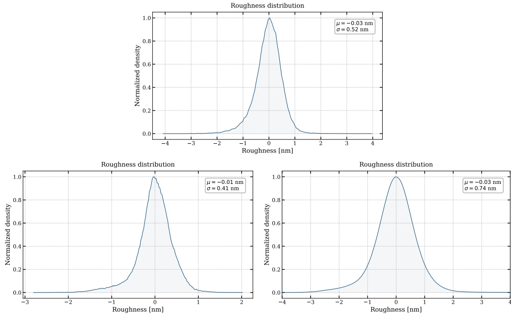
Figure 12: Surface roughness distribution obtained through AFM. It can be seen that most of the defects are below the 1 nm range. Furthermore, the mean ( \mu ) is close to zero, confirming that the surface is uniform.
