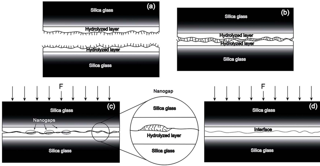
Figure 4: Effects of pressure in the bonding process. Interface voids can be prevented by applying forces in the direction perpendicular to the interface. From [20]
