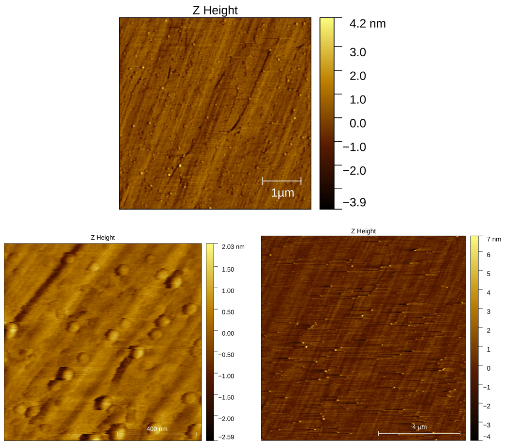
Figure 10: 2D Surface images obtained through AFM in three different parts of the pristine Nanoquartz disk's surface.
