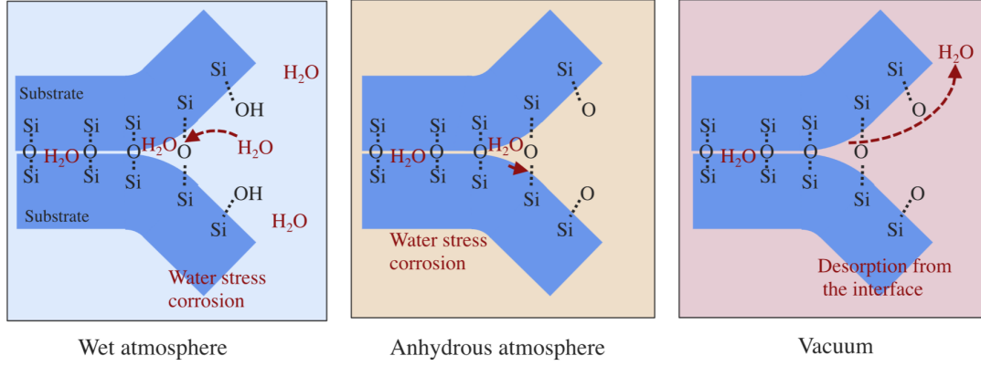
Figure 7: Schematic representation of water stress corrosion at the hydrophilic bonding interface during debonding under controlled atmospheres. Left: wet atmosphere showing ambient water attack on Si–O–Si bonds. Center: anhydrous (dry) atmosphere with reduced water availability. Right: vacuum conditions with partial desorption of interfacial water. Adapted from [27].
