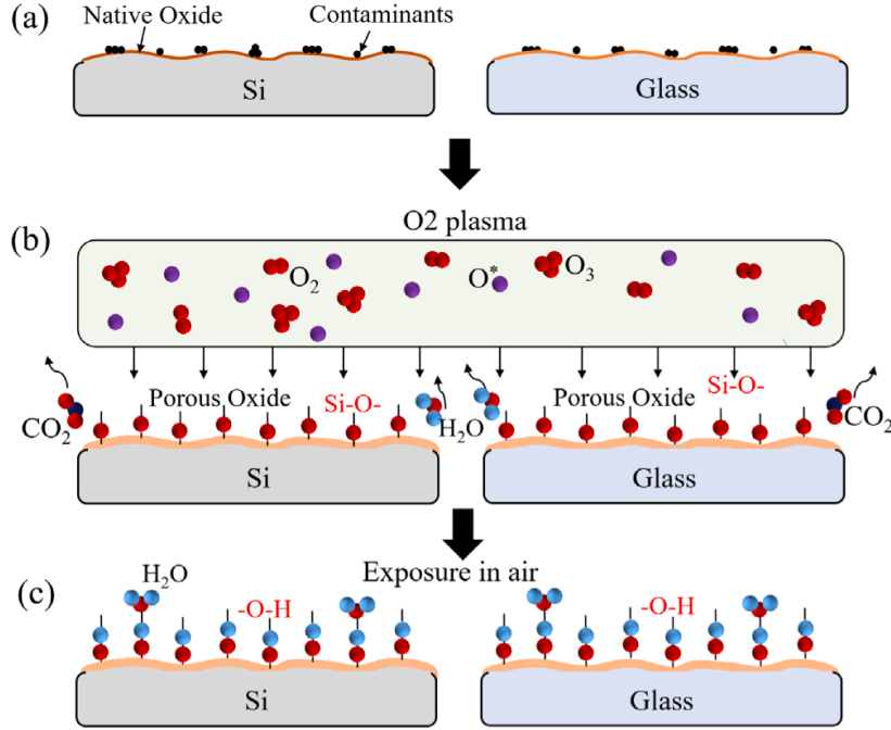
Figure 2: Effects of plasma treatment on silica surfaces. Plasma helps to remove contaminants while increasing the number of available silanol groups. Adapted from [14]
