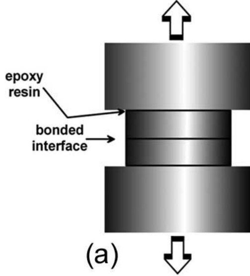
Figure 8: Schematic diagram of the tensile test setup for bonding strength measurement. The bonded wafer pair is glued to metal fixtures and subjected to perpendicular tensile force. Adapted from [7].
