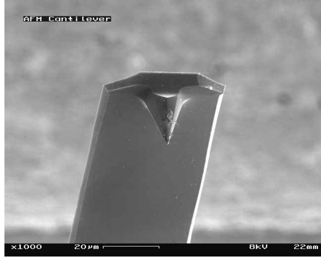
Figure 9: View of cantilever in Atomic Force Microscope (magnification 1000x) [33]
