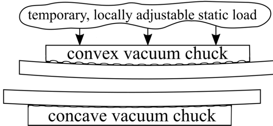
Figure 3.5: Pressure plate geometry described by Birckigt et al. [39]. The curved profiles guide contact front propagation outward from the center, reducing the probability of interface void formation.
