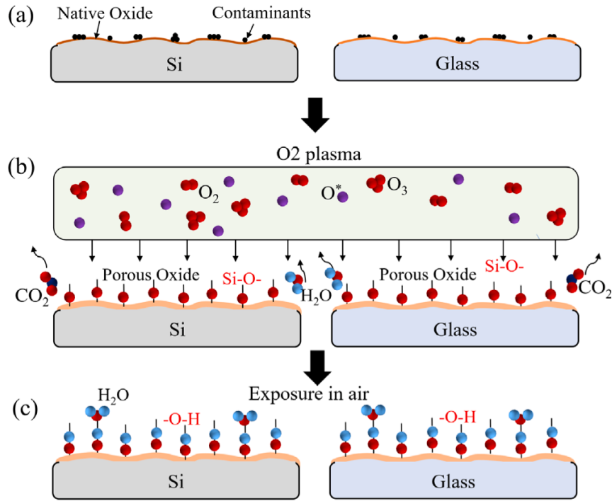
Figure 3.2: Effects of plasma treatment on silica surfaces. Plasma removes contaminants and increases the density of available silanol groups. Adapted from [31].
