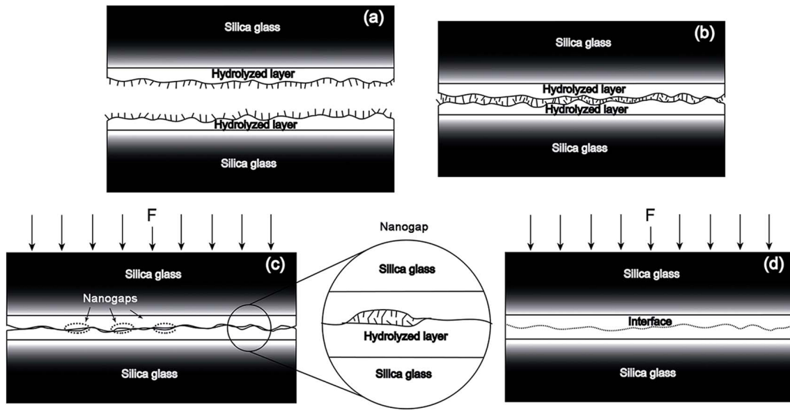
Figure 3.4: Effect of applied pressure on the bonding process. Forces perpendicular to the interface suppress void formation by closing residual gaps between surface asperities. From [36].
