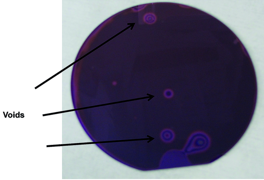
Figure 4.1: Newton rings being formed on the interphase of a SiN-glass wafer. From [41].
