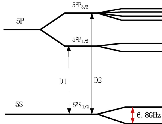
Figure 4.8: Energy level diagram showing the D1 and D2 transitions in an alkali metal atom. From [54]
