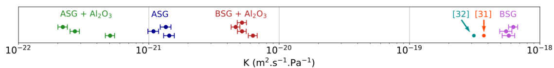
Figure 3.16: Comparison of the permeability constant K across uncoated borofloat, uncoated aluminosilicate, Al 2 O 3 -coated borofloat, and Al 2 O 3 -coated aluminosilicate glasses. From [34].
