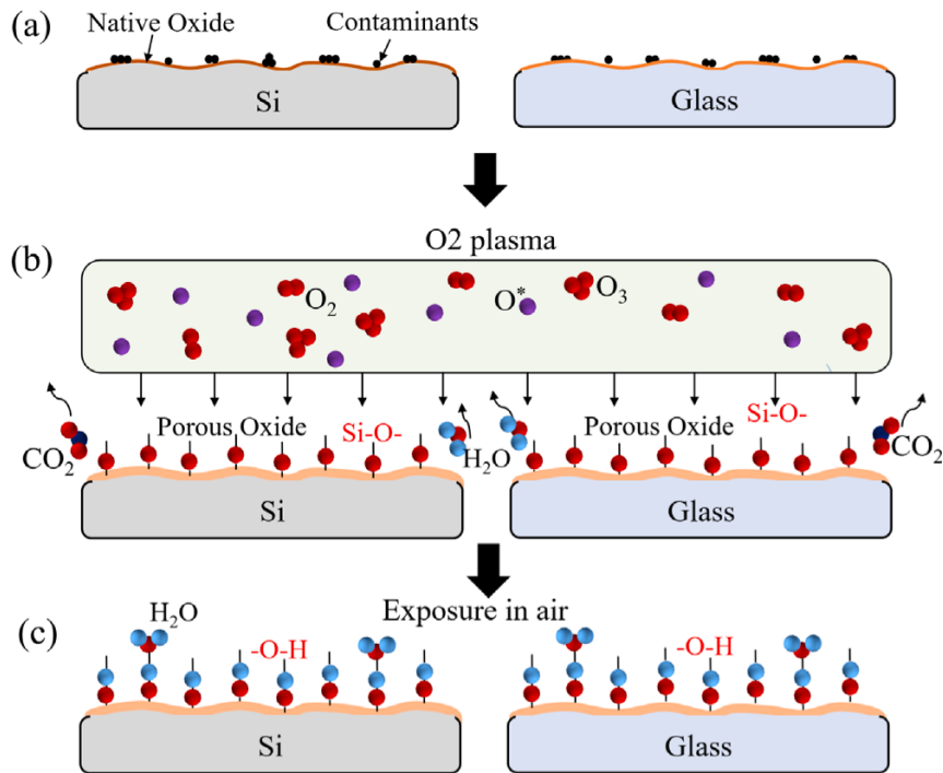
Figure 3.6: Effects of plasma treatment on silica surfaces. Plasma removes contaminants and increases the density of available silanol groups. Adapted from [53].
