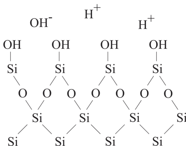
Figure 3.4: Schematic representation of a hydroxylated/hydrophilic surface. From [43].
