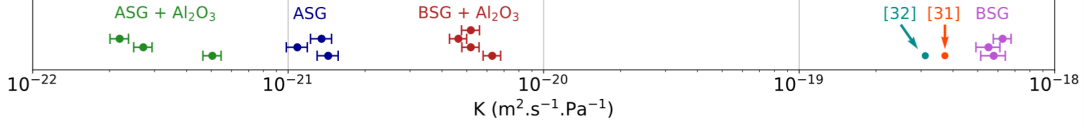
Figure 6: Comparison of the permeability constant K across uncoated borofloat, uncoated aluminosilicate, \text{Al}_2\text{O}_3 -coated borofloat, and \text{Al}_2\text{O}_3 -coated aluminosilicate glasses. From [25].
