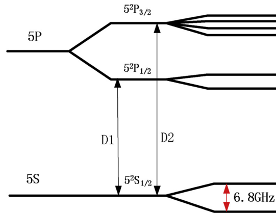
Figure 5: Energy level diagram showing the D1 and D2 transitions in an alkali metal atom. From [20]
