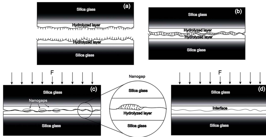
Figure 3.10: Effect of applied pressure on the bonding process. Forces perpendicular to the interface suppress void formation by closing residual gaps between surface asperities. From [60].
