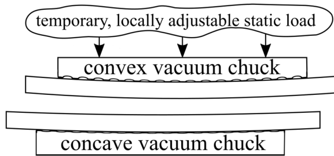
Figure 3.11: Pressure plate geometry described by Birckigt et al. [64]. The curved profiles guide contact front propagation outward from the center, reducing the probability of interface void formation.
