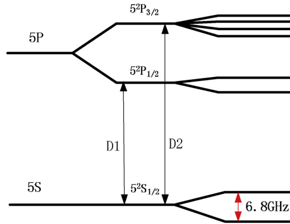
Figure 4.11: Energy level diagram showing the D1 and D2 transitions in an alkali metal atom. From [74]
