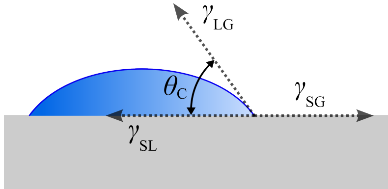
Figure 4.5: A diagram that shows the contact angle and interphase-energy between 3 phases (gas, liquid, solid). From [59].
