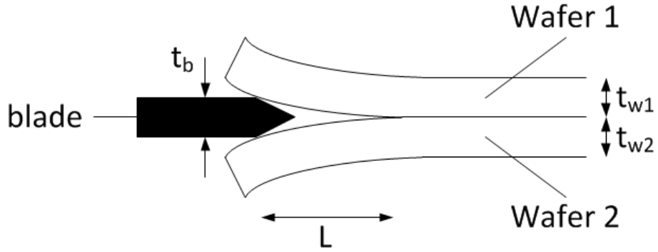
Figure 4.8: Illustration of the razor blade method. A razor blade is inserted between the bonded surfaces in order to quantify the bonding energy between them. From [64].
