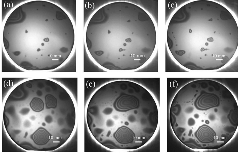
Figure 4.7: Examples of Newton rings formed in the interphase of Si/Si wafers. From [62].
