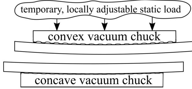
Figure 3.7: Pressure plate geometry described by Birckigt et al. [55]. The curved profiles guide contact front propagation outward from the center, reducing the probability of interface void formation.
