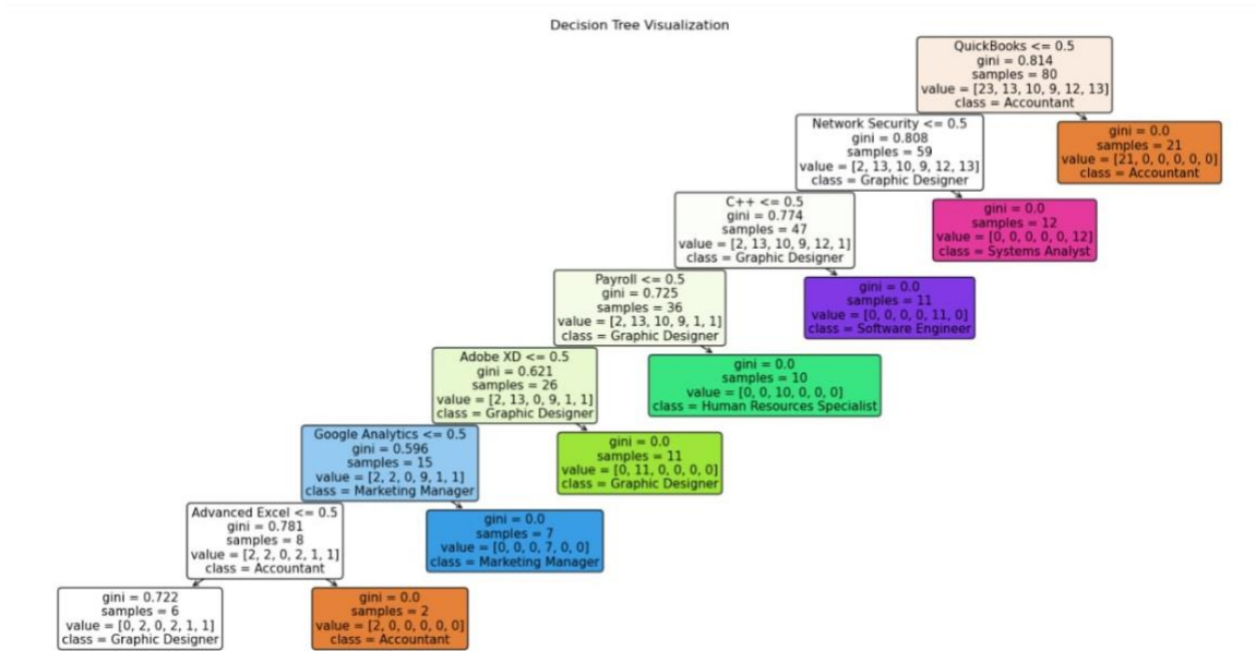
Figure 7: Decision Tree Visualization
