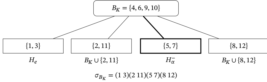
Figure 9: The concrete star of the dodecaphasic flag. Each line indicates the union of the central four-element set with the pair at its endpoint; the thick line marks the hexad also selected by the signs preceding the carry of \alpha . The four pairs exhaust the eight outer positions.
