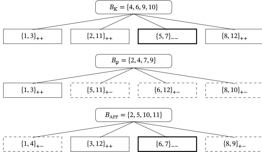
Figure 10: Comparison of the three stars. Each connection represents the union of the upper four-subset with one pair; the twelve complete hexads appear in Table 12. Thick outlines indicate negative pairs and dashed outlines mixed pairs. The connections represent incidence.
