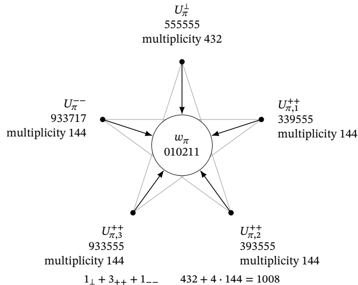
Figure 11: The five regions of \pi in a pentadic arrangement. Each position preserves its multiplicative signature and multiplicity; the radial arrows represent the common projection \Psi(U) = 010211 . The star-shaped outline organizes the five positions of the chart. Their realization in the five Witt octads is performed through regional alignment and the 4 + 1 decomposition in the text.
