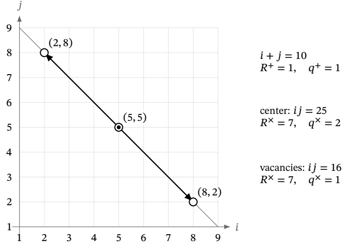
Figure 8: Electronic center and conjugate vacancies in the APP chart. The diagonal is the additive fiber \mathcal{F}_{10} ; the center is the fixed point of (i, j) \mapsto (10 - i, 10 - j) . The two shifts of magnitude 3 preserve the sum and product residue and reduce the multiplicative quotient by one unit. The arrows represent deformations on the fiber.
