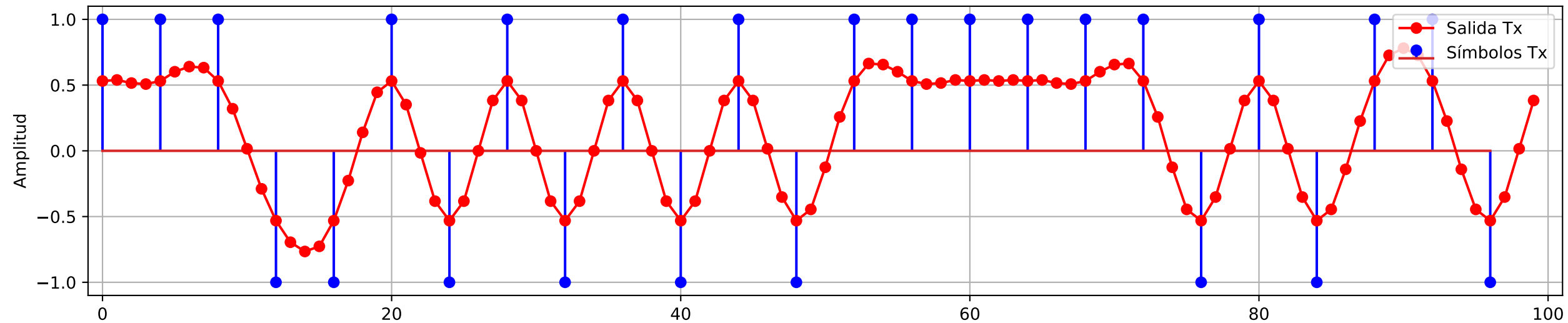
Transmisor (I)
