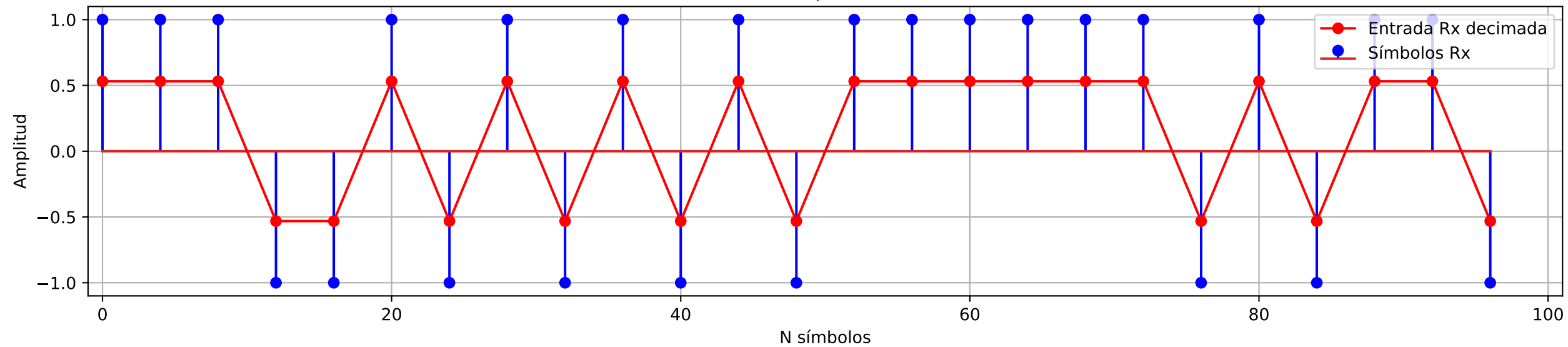
Receptor (I)
