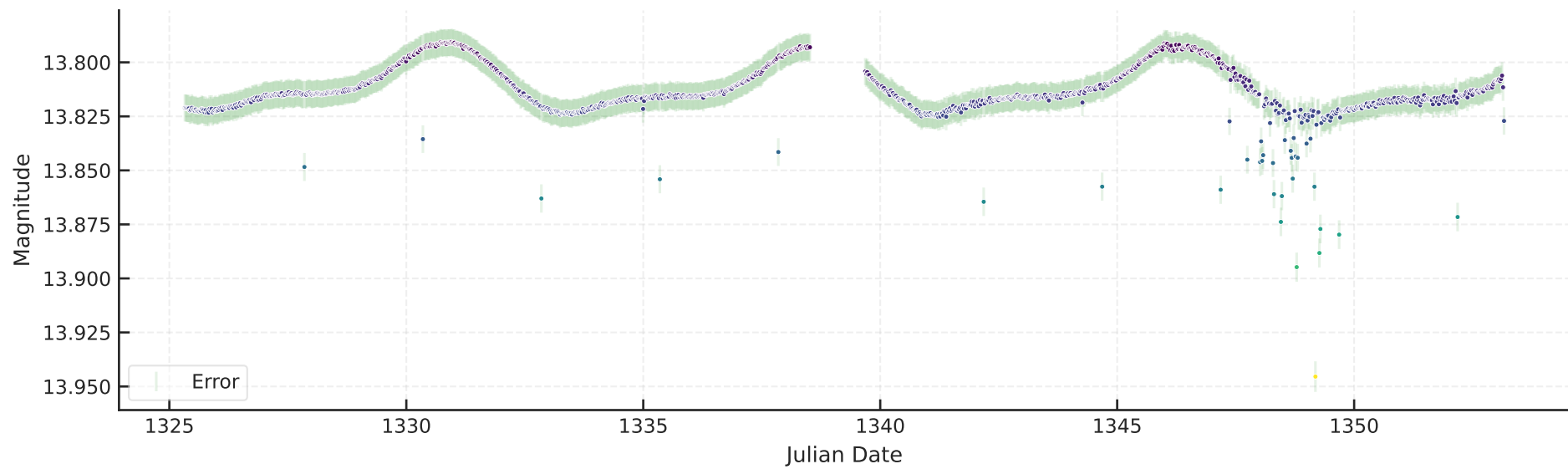
TESS 270304671 ACV - Median after CBV
