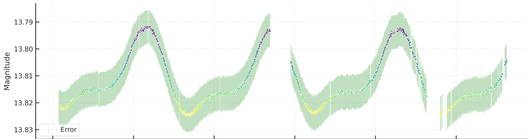
TESS 270304671 ACV - Median after CBV
