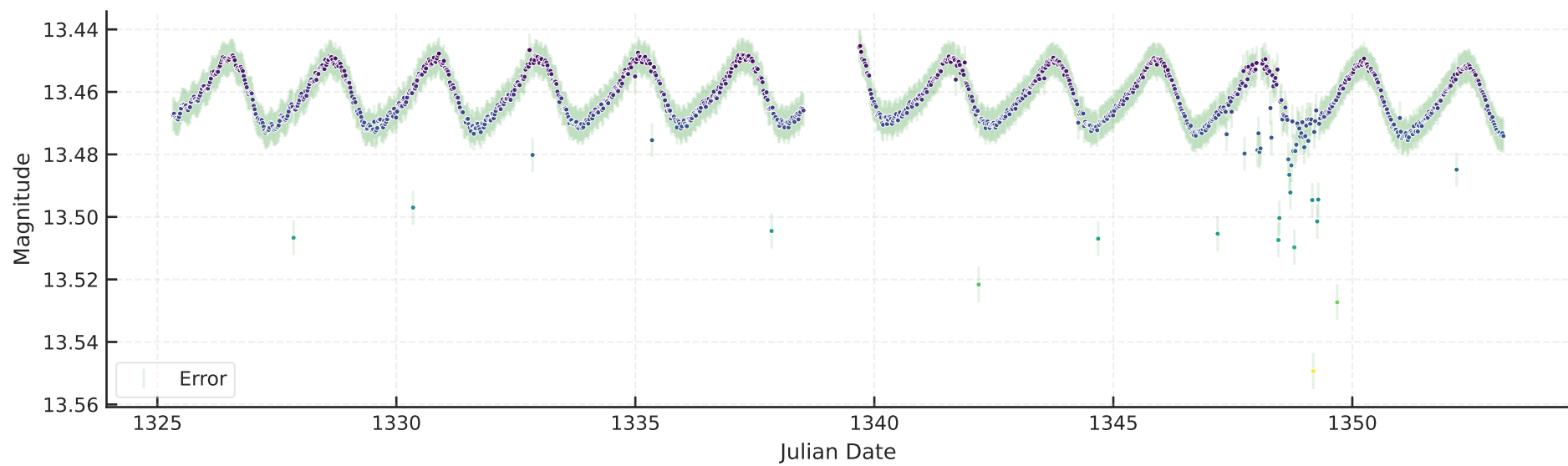
TESS 92705248 ACV - Median after CBV
