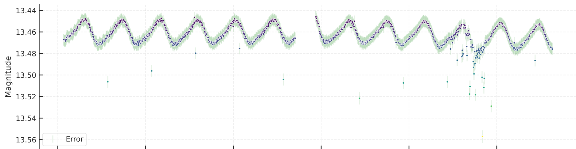
TESS 92705248 ACV - Outlier cleaned
