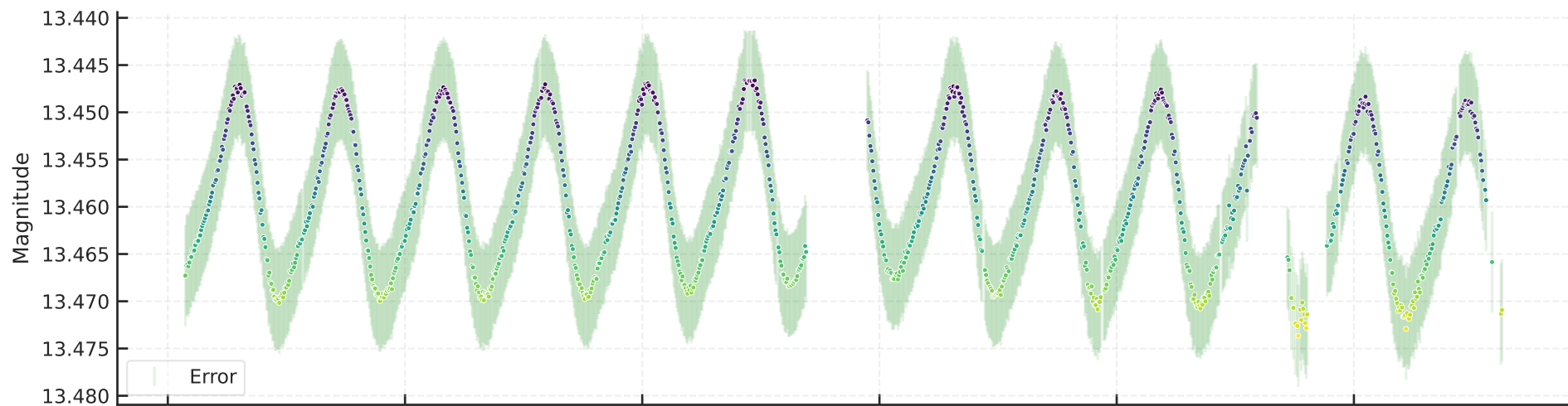
TESS 92705248 ACV - Median after CBV
