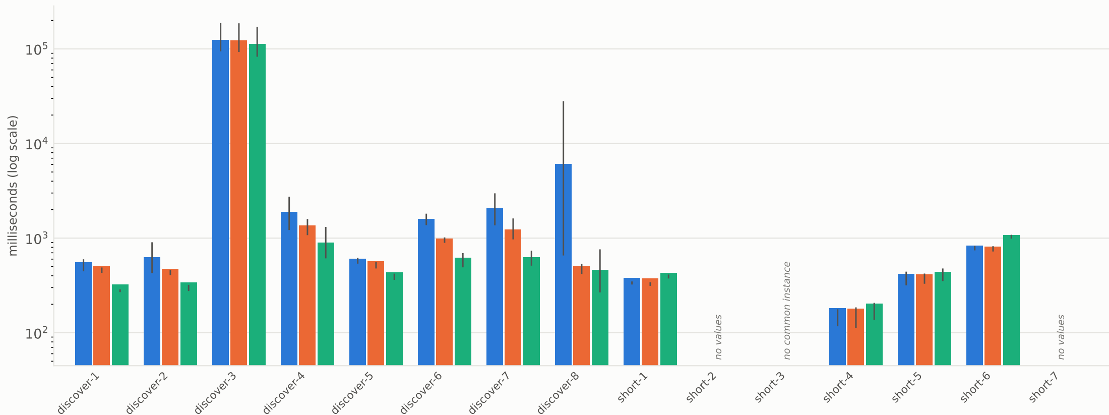
Time to first result per query template
