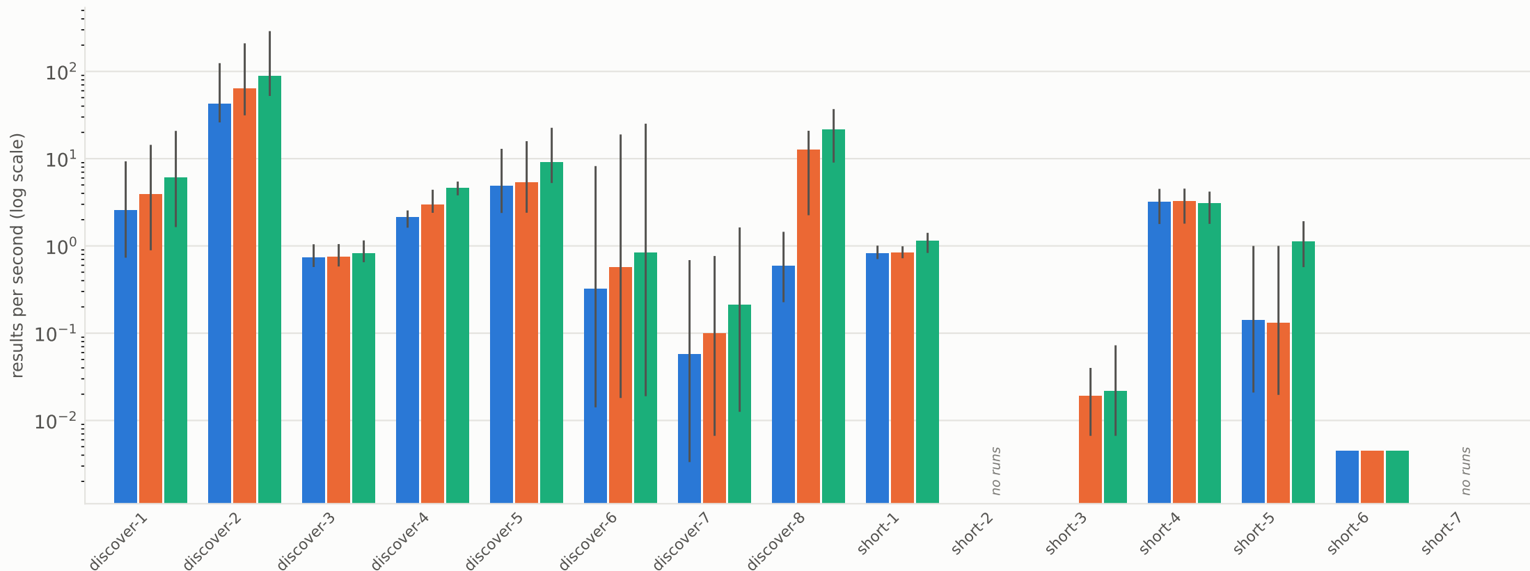
Result throughput per query template
