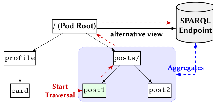
Figure 1: Data coverage overlap and traversal dynamics. Execution starts at post1, traversing up the LDP hierarchy until it discovers the SPARQL endpoint at the root. Because this endpoint acts as an alternative view aggregating the same posts already being traversed, the engine retrieves duplicate data.
