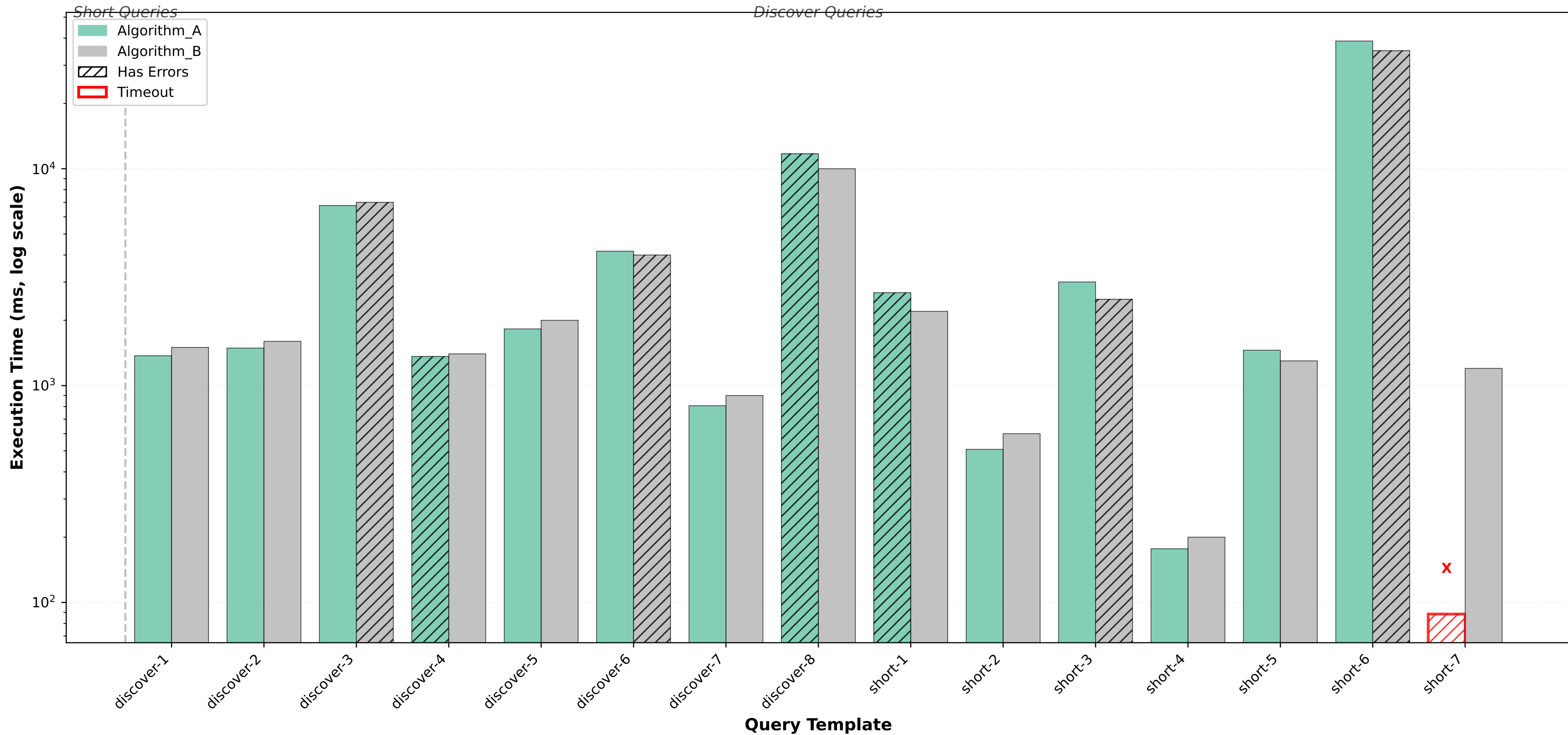
Algorithm Performance Comparison Across Query Templates
