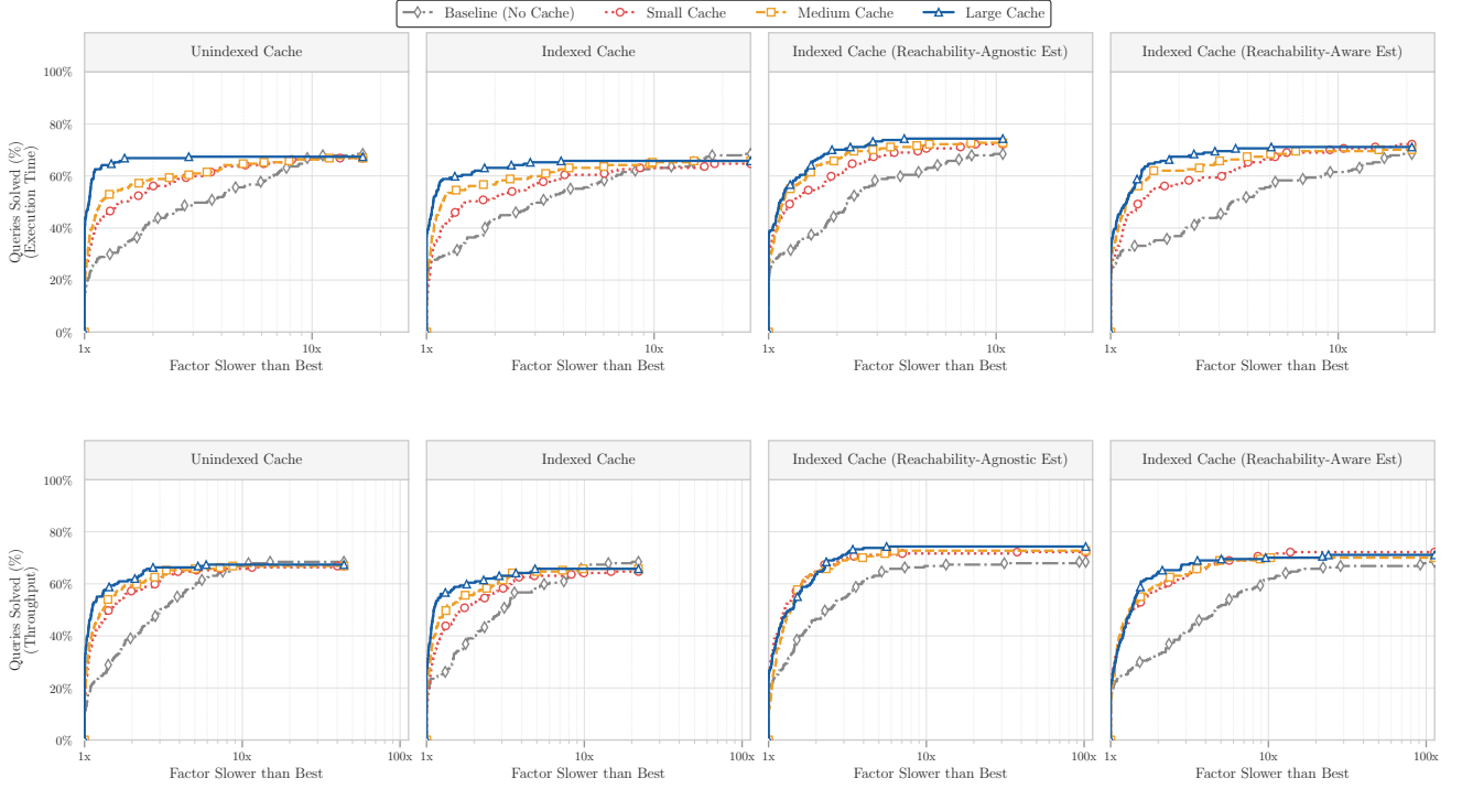
Figure 2: Performance profiles of the LRU-based unindexed and indexed triples cache. The y-axis shows the percentage of queries executing within a factor ( x -axis) of the fastest algorithm. Curves closer to the top-left indicate better overall performance. The y-intercept ( x = 1 ) shows how often an algorithm is the outright fastest, while the rightward trajectory demonstrates robustness (e.g., x = 2, y = 80\% means 80% of queries execute within twice the fastest time). From the figure, we observe that all caching-based approaches outperform the no-cache baseline.
