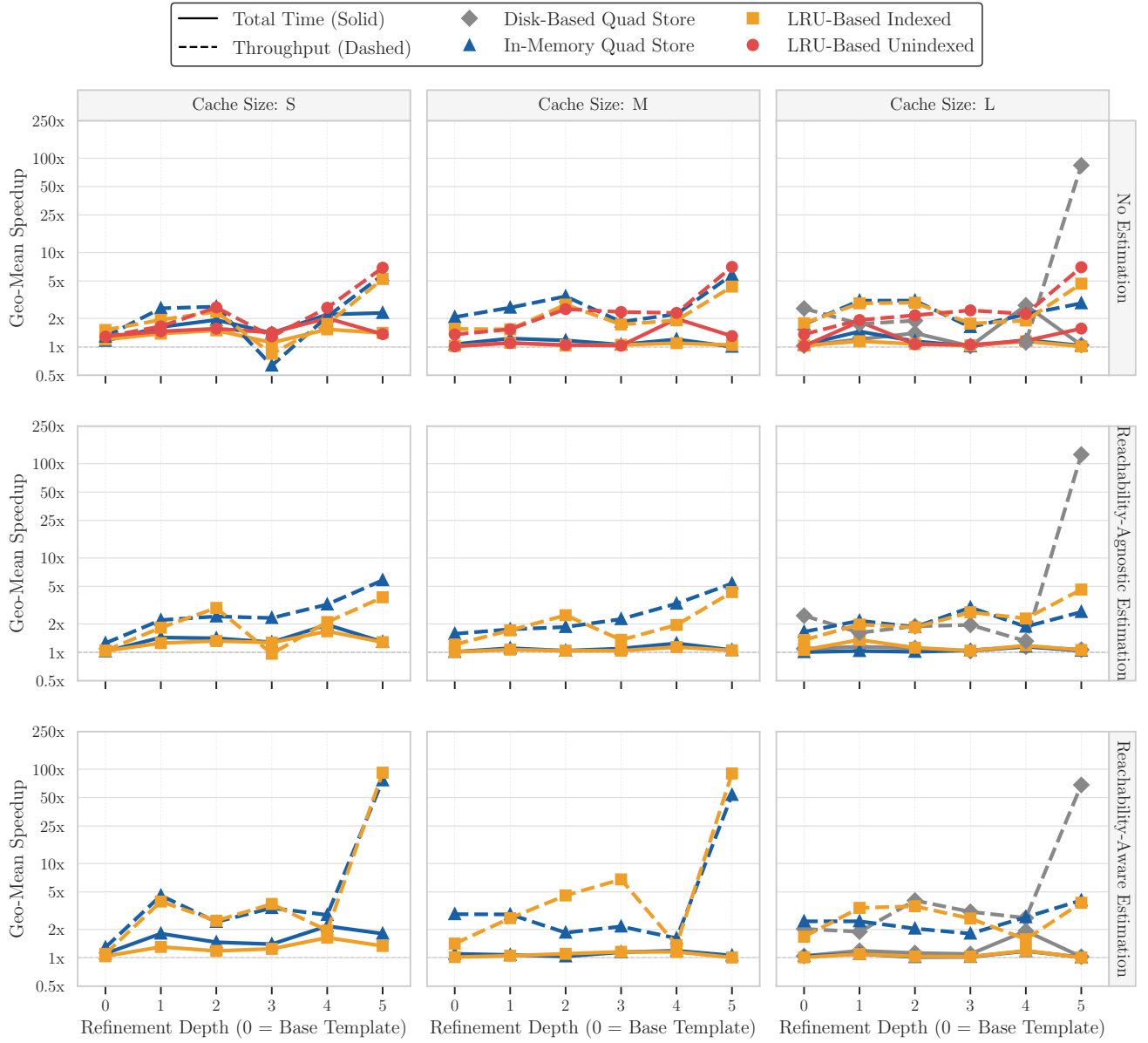
Figure 6: Geometric mean speedup of total execution time (solid lines) and query throughput (dashed lines) relative to the no-cache baseline. Results are faceted by cardinality estimation strategy (rows) and cache capacity (columns). The Reachability-Aware Estimation row and Large cache column utilize a logarithmic y-axis to accommodate significant performance gains at higher refinement depths.
