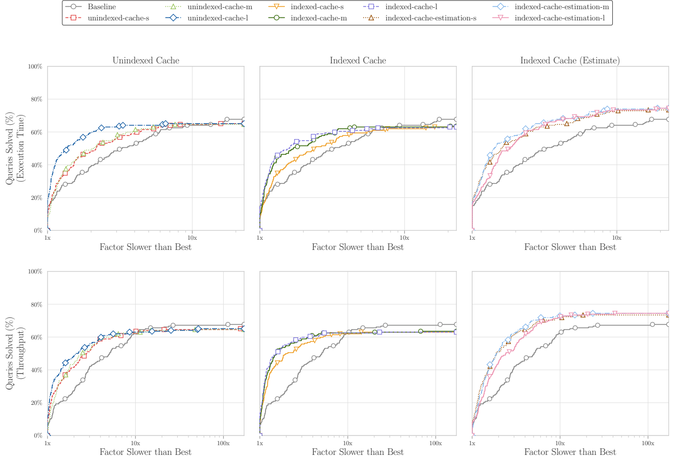
Figure 2: Performance profiles of the tested cache algorithms. The y-axis shows the percentage of queries executing within a factor ( x -axis) of the fastest algorithm. Curves closer to the top-left indicate better overall performance. The y-intercept ( x = 1 ) shows how often an algorithm is the outright fastest, while the rightward trajectory demonstrates robustness (e.g., x = 2, y = 80\% means 80% of queries execute within twice the fastest time). From the figure, we observe that all caching-based approaches outperform the no-cache baseline.
