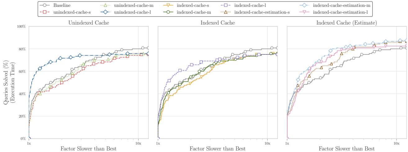
Figure 6: Performance profile of the tested cache algorithms on random query sequences. The y-axis shows the percentage of queries that execute within a given performance factor (x-axis) of the fastest algorithm for that query.
