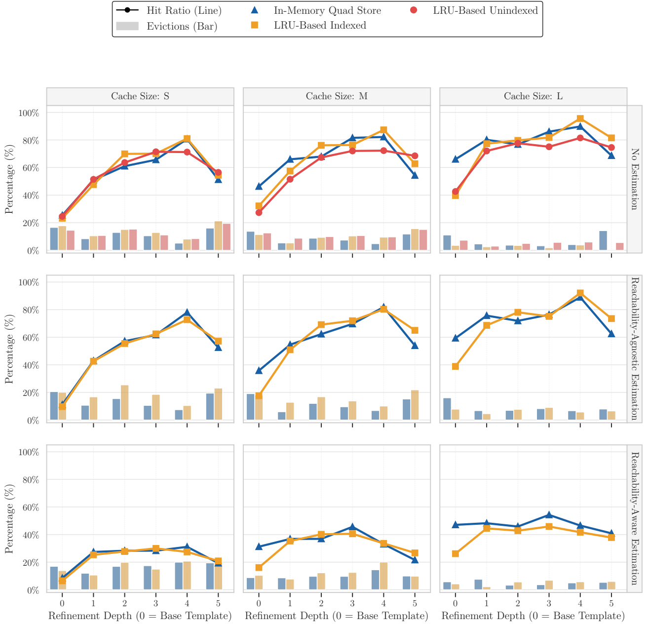
Figure 5: Cache hit ratio and eviction percentage across refinement depths (0 to 5). The grid separates configurations by cardinality estimation strategy (rows) and cache capacity (columns). Line plots denote the cache hit ratio, while the shaded background bars represent the percentage of cache capacity evicted during the sequence.
