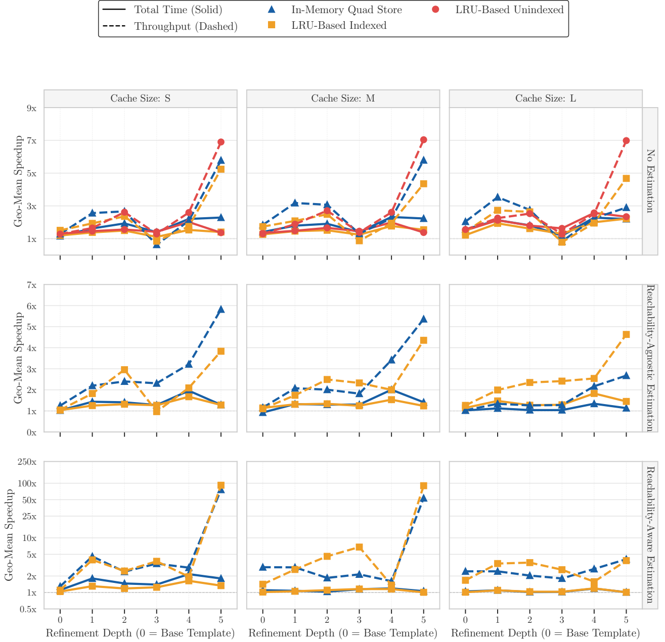
Figure 6: Geometric mean speedup of total execution time (solid lines) and query throughput (dashed lines) relative to the no-cache baseline. Results are faceted by cardinality estimation strategy (rows) and cache capacity (columns). The Reachability-Aware Estimation row utilizes a logarithmic y-axis to accommodate significant performance gains at higher refinement depths, whereas the other strategies cap linearly at 20x.
