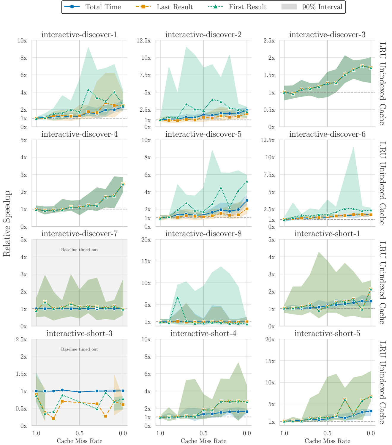
Figure 10: Performance of LRU-based unindexed cache across all query templates. The y-axis shows the mean speedup relative to a baseline with a 0% hit rate. Shaded regions denote the 90th percentile
