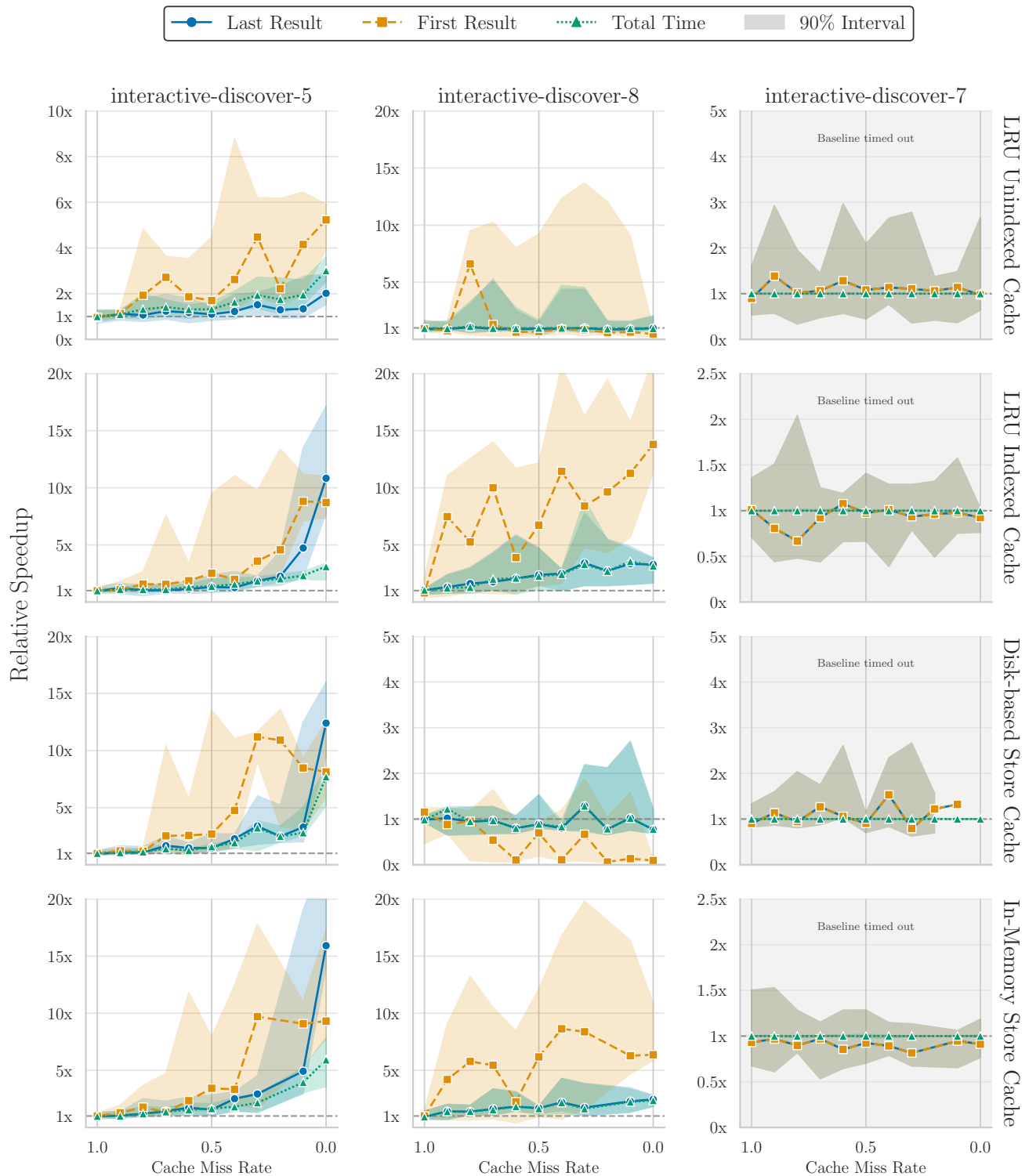
Figure 7: Performance of LRU-based unindexed, LRU-based indexed, In-memory store, and Disk-based store caches across representative query templates. The y-axis shows the mean speedup relative to a baseline with a 0% hit rate. Shaded regions denote the 90th percentile
